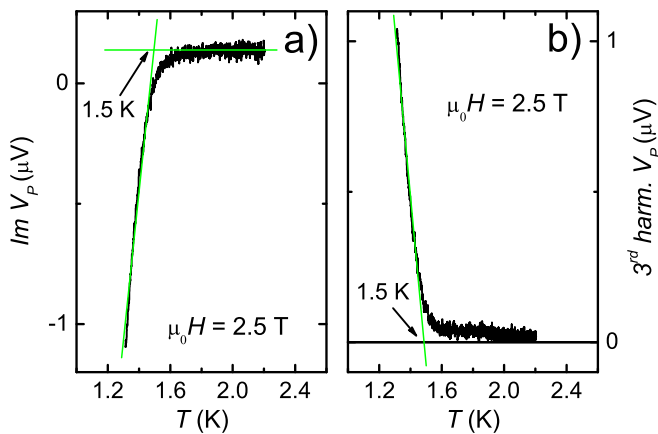
FIG. 4: Temperature dependence of the imaginary part (a) and the third harmonic (b) of the pickup voltage measured in the paramagnetic part of a dHvA oscillation at the beat node for 2.5 T with 40 \mu T modulation amplitude.
