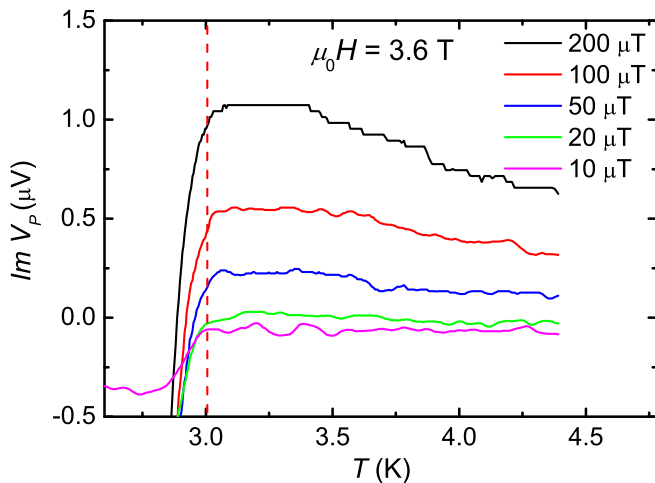
FIG. 2: Temperature dependence of the imaginary part of the pickup voltage for several modulation amplitudes at the paramagnetic part of a dHvA oscillation at the beat antinode at 3.6 T. The dashed line indicates the critical temperature T_c = 3.0 K where the Condon domain phase is entered when lowering the temperature.
