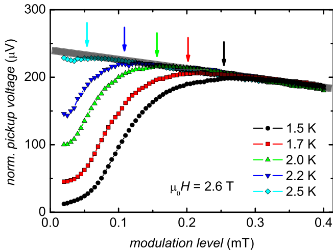
FIG. 7: Normalized pickup voltage as function of modulation level for several temperatures in the center of the dHvA oscillation at 2.6 T corresponding to the center of a needle-like stripe like shown in Fig. 6. The arrows indicate the chosen hysteresis sizes h_m .
