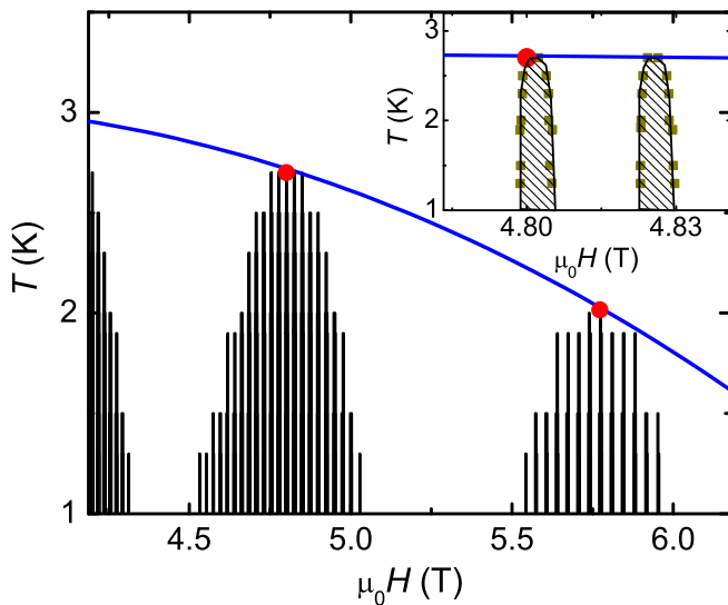
FIG. 6: Expanded view of Fig. 5 around the beat maximum at 4.8 T showing the beating substructure of the phase diagram. The slight steps in the envelope of the height of the needle-like stripes results from the limited number of measured temperatures. The expanded view in the inset shows the detailed phase diagram in two successive dHvA periods obtained by field sweeps at constant T . The larger round circles are obtained by T -sweeps at constant H .
