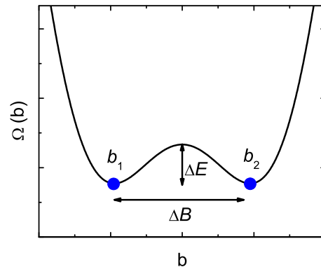
FIG. 9: Schematic representation of the Lifshitz-Kosevich potential in the CDS showing two minima corresponding to the domain states with the inductions B_1 = \mu_0 H + b_1 and B_2 = \mu_0 H + b_2 and a potential barrier \Delta E in the domain wall between the domains.
