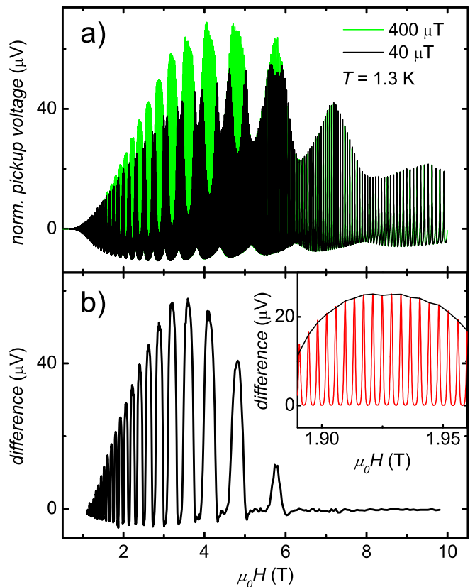
FIG. 1: (a) Pickup voltage normalized on the modulation level for high ( 400 \mu T) and low ( 40 \mu T) modulation level at 1.3 K. Due to hysteresis in the CDS the pickup voltage decreases if the modulation level is of the order or smaller than the hysteresis loop width. (b) Envelope of the difference between both curves of Fig. 1(a) showing the field regions where Condon domains exist for non-zero difference. The inset shows an expanded view of the difference signal with the appearance of hysteresis in a part of each dHvA period.
