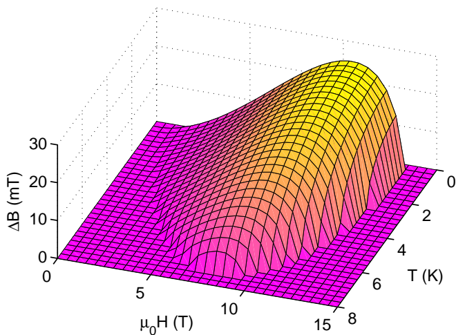
FIG. 10: Calculation of the induction difference \Delta B between the domains as a function of H and T for a Dingle temperature T_D = 2.0 K.
