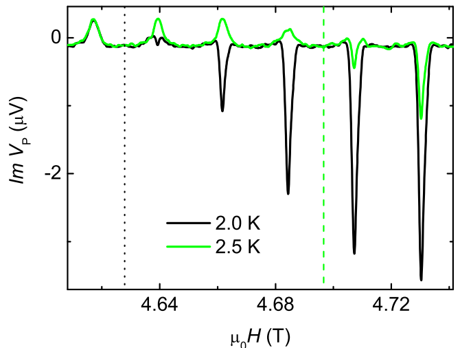
FIG. 3: Field dependence of the imaginary part of the pickup voltage measured at 2.0 K and 2.5 K with 40 \mu T modulation amplitude. The steeply increasing negative amplitude is caused by the hysteresis in the CDS. The vertical dotted lines indicate the transition field to the CDS for 2.0 and 2.5 K.
