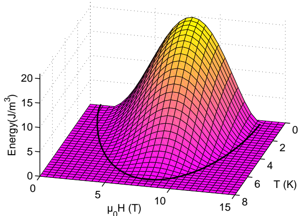
FIG. 11: Numerical calculation of the energy barrier \Delta E between the domains with the respective inductions B_1 and B_2 as a function of H and T for a Dingle temperature T_D = 2.0 K. The solid line indicates the Condon domain phase boundary using the 'cylinder' model of Ref. 15.
