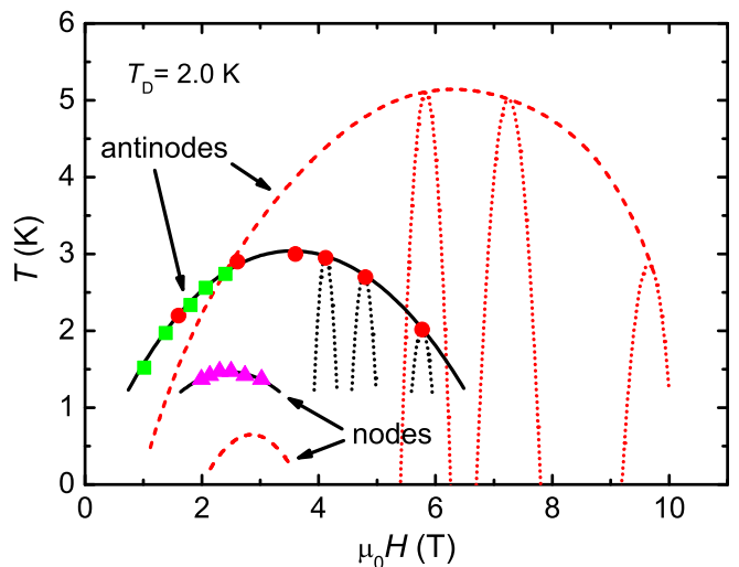
FIG. 5: Phase diagram in the (H, T) plane for beryllium. Scatter points indicate the position of the phase boundary at beat nodes and antinodes determined by temperature sweeps (circles and triangles) like in Figs. 2 and 4 and by field sweeps (squares) like in Fig. 3. The solid lines are guiding lines of the phase boundary for beat nodes and antinodes, respectively. The dashed lines show for comparison the recent theoretical calculation of Ref. 6,15. The dotted lines indicate the envelope of the beating substructure of the phase diagram shown in detail in Fig 6.
