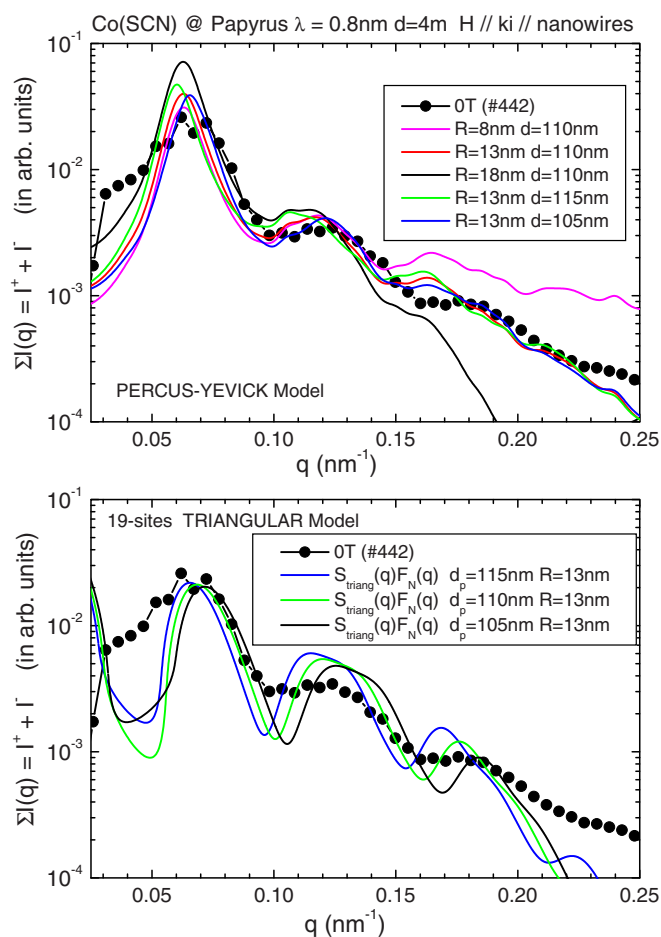
FIG. 4. (Color online) (a) SANS data ( \lambda = 0.8 nm) compared with a fitted SANS model including a Percus-Yeivick structure factor S_{\text{PY}}(q) and a Bessel-type expression for the nuclear form factor F_N(q) . The best agreement is found for d_p = 110 nm and R = 13 nm (red line). For all fits, \eta is fixed to 0.5. (b) Triangular array model [Eq. (21)] with R = 13 nm fixed and varying inter-pore distance d_p . The agreement is correct regarding peak positions but rather poor regarding lineshapes.
