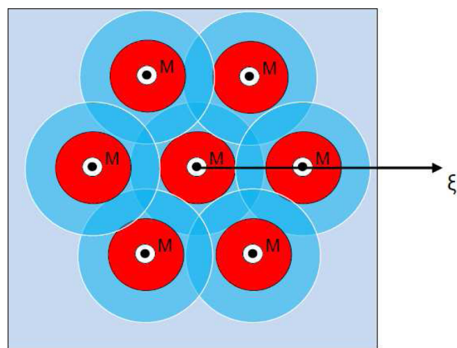
FIG. 9. (Color online) Triangular array of nanowires with homogeneous magnetization inside the core (in red) and dipolar field intensity (in blue). The dipolar field creates a neutron scattering contrast with the non-magnetic matrix. The axis \xi will meet different dipolar field profile depending on its relative orientation. The data obtained will then correspond to a profile average.
