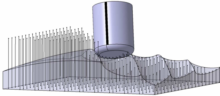
Fig. 1 3D surface topography simulation in 5 axis-milling
