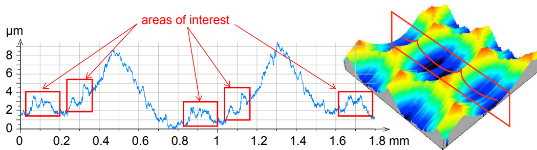
Fig. 3 Actual defects in the bottom of the valleys
