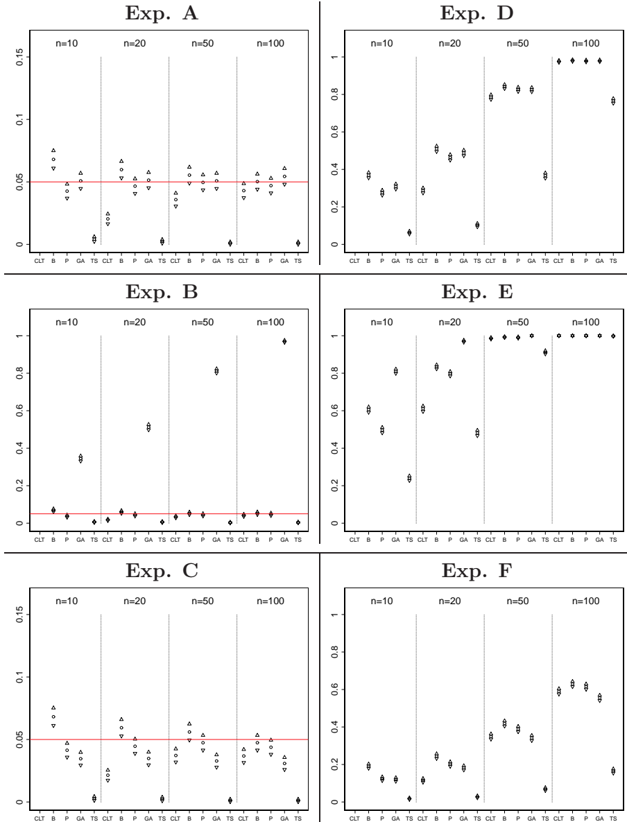
Figure 1 – Estimated sizes and powers for various numbers of trials n , all the tests being performed with a level \alpha = 0.05 . The circles represent the percentage of rejection on 5000 simulations for each method, the triangles represent the corresponding endpoints of a 95% confidence interval. The corresponding experiments are described in Section 5.1.2.
