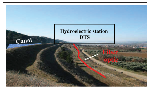
Figure 4. Real dike of EDF bounding the feed canal of the hydroelectric station: illustration of location of optical fiber at the toe of the dike.
