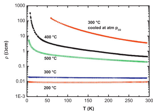
Fig. 7. Electrical resistivity curves as a function of temperature for the \text{In}_2\text{O}_3 films grown at 200, 300, 400, 500 °C and 300 °C under cooling at atmospheric \text{P}_{\text{O}_2} .
