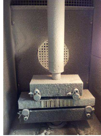
Figure 6: Flexural load of a sandwich specimen at -60^{\circ}\text{C}
