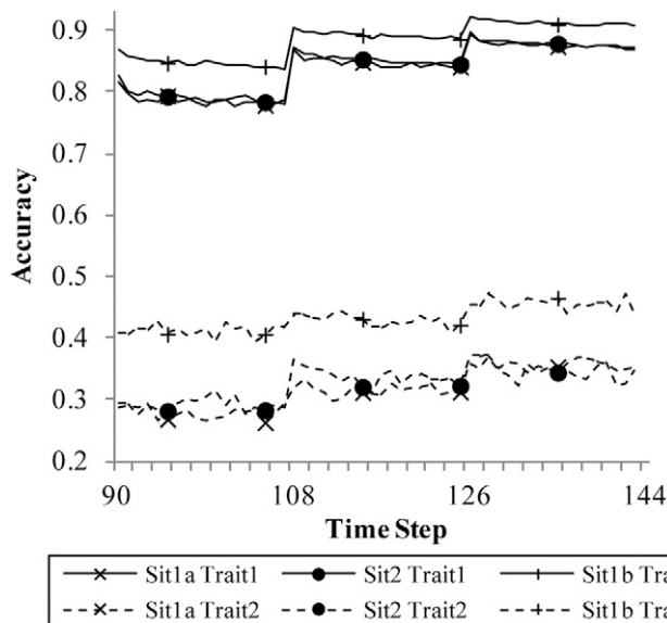
Figure 3. Evolution of the accuracy of genomic EBV of candidates available for selection at each time step, considering different lengths of simulated genome and different values for the scaling factor applied to the size of the training population. The initial QTL density was 30 QTL/M for each trait, and heritabilities of Trait 1 and Trait 2 were 0.4 and 0.2, respectively. The results are averages of 30 replicates: Sit1a, 5 pairs of 100-cM chromosomes applying a scaling factor of 1/6; Sit1b, 5 pairs of 100-cM chromosomes applying an inadequate scaling factor of 1/3; and Sit2, 10 pairs of 100-cM chromosomes applying a scaling factor of 1/3.
