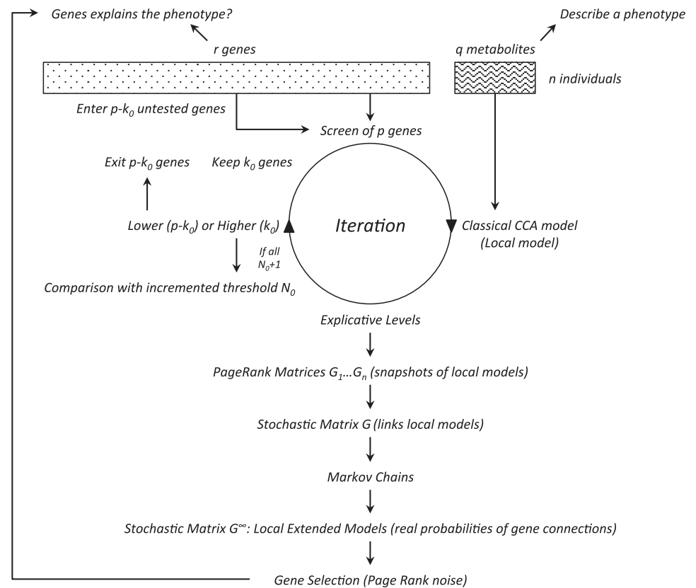
Fig. 1. Principle of the gene selection method.
