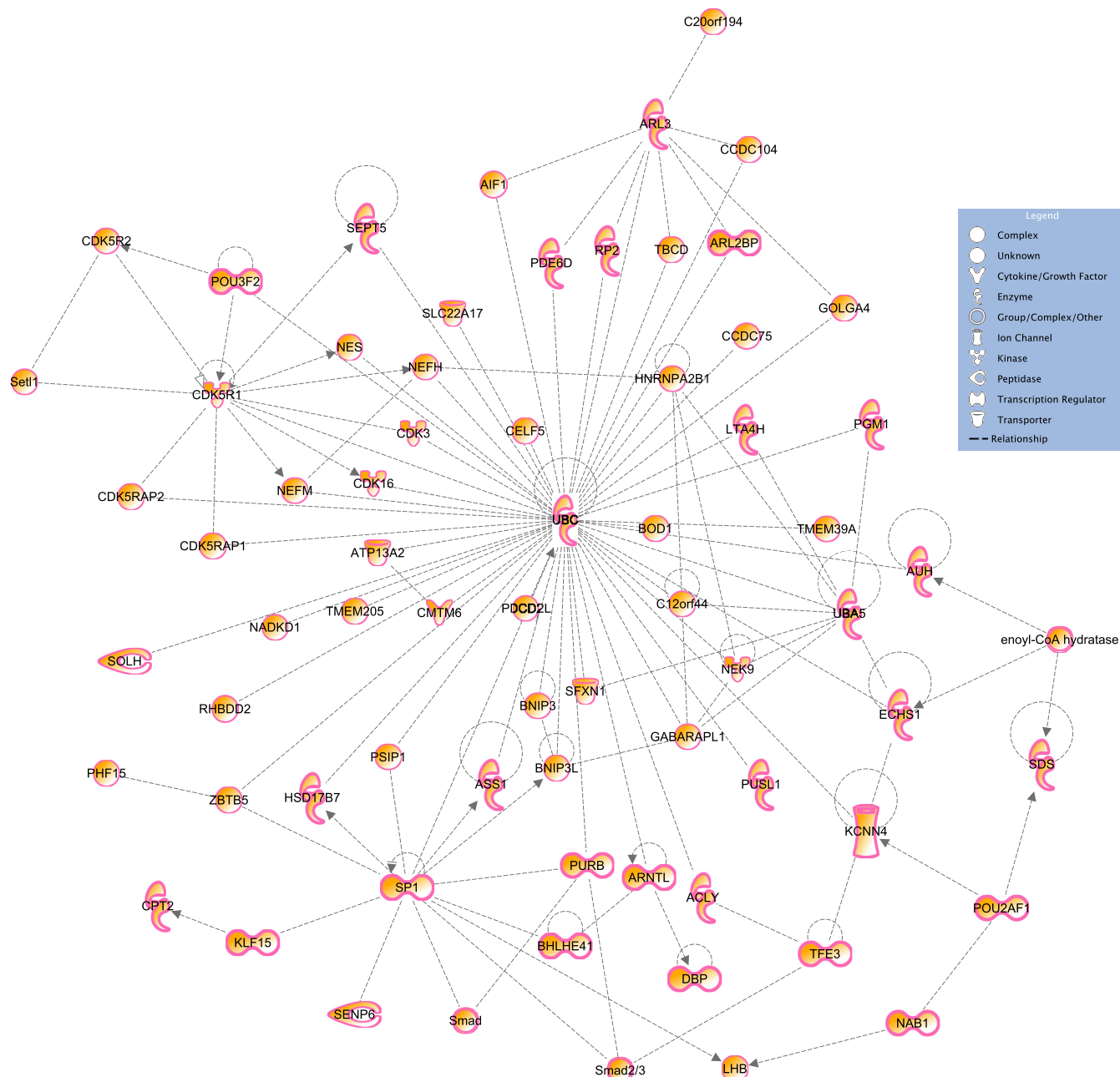
Fig. 7. We compared gene networks related to “cell morphology,” involving both algorithm-specific genes and genes in common between sPLS and algorithm analyses. These networks come from the LiverTox datasets and appear complementary. Gene IDs are those recognized by the IPA software. Displayed networks correspond to those from Fig. 6, namely: algo-specific/network 1 vs. algo-sPLS-shared/network 8.
