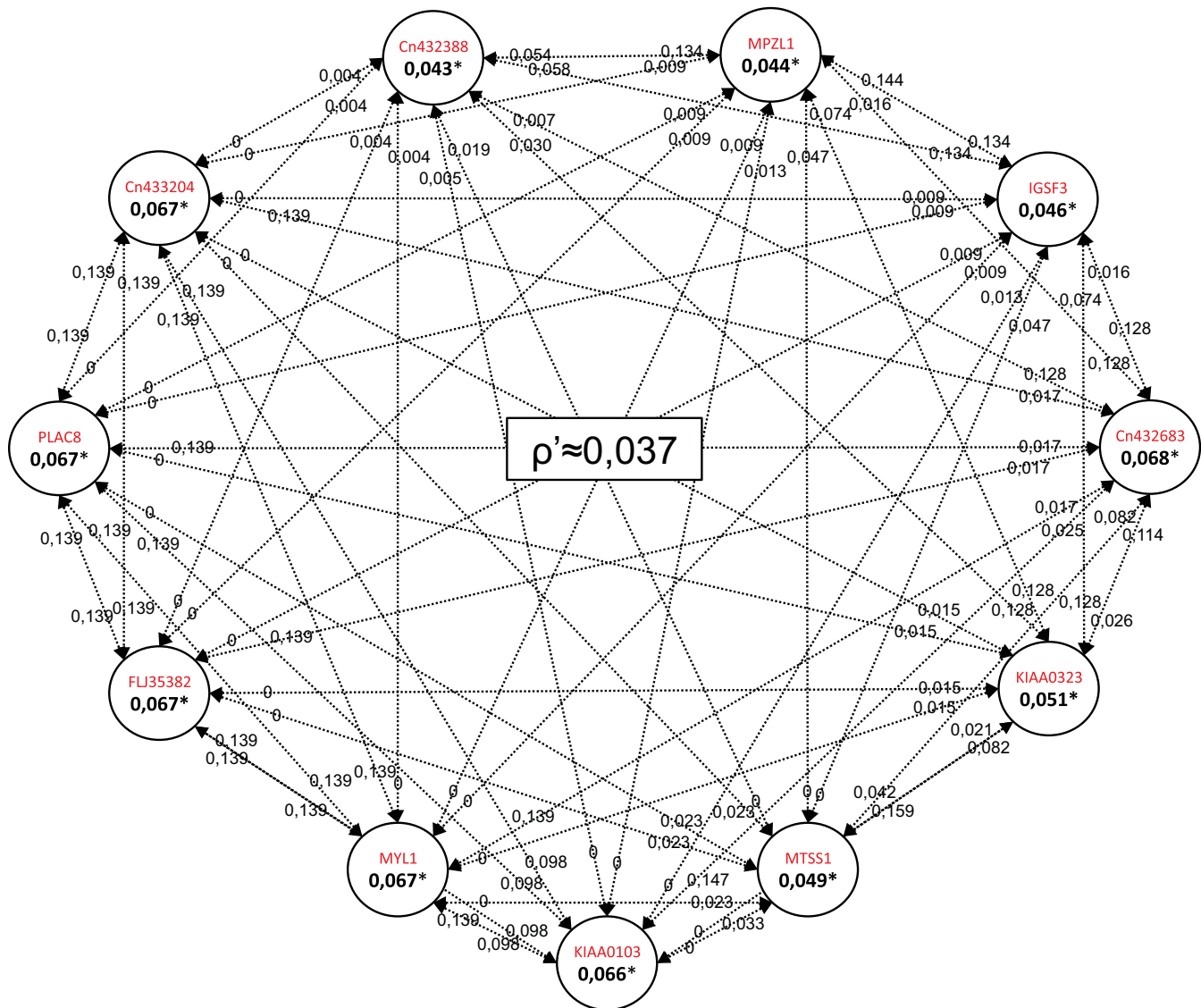
Fig. 5. Weighted Markovian graph of the major local extended model (LEM) issued from the canonical correlation analysis (CCA)-based heuristic algorithm. The stochastic matrix G including the genes association probabilities was computed. G elevated to a certain power is a diagonal block-wise matrix of which the diagonal submatrices are corresponding to genes of the same LEM. The sequence of the successive powers of G was iterated in order converge each column of the submatrices to a nearly constant vector as expected in the Markovian theory (see R program). It was sufficient to compute G^{10} . Then, we can exclude nonessential and nonsignificant genes from the LEM. Here are shown the 11 selected genes (among 27) with a column mean P verifying P > \rho' ( \rho' is the threshold of PageRank noise). They are presented inside circles and are labeled with their own probability extracted from G^{10} (*). Those probabilities represent the importance of the gene in the LEM. Probabilities on the connective arrows (dotted lines) are issued from the matrix G . For simplicity extra connections with nonessential or nonsignificant genes are not represented.
