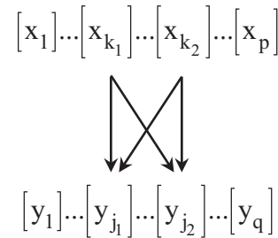
Fig. 2. Directed bipartite graph with respect to the pairs of values (\xi_i, \eta_i) , where x_k ( k from 1 to p ) is the gene sequence; y_j ( j from 1 to q ) is the metabolite sequence. An arrow represents the association between a gene and a metabolite.
