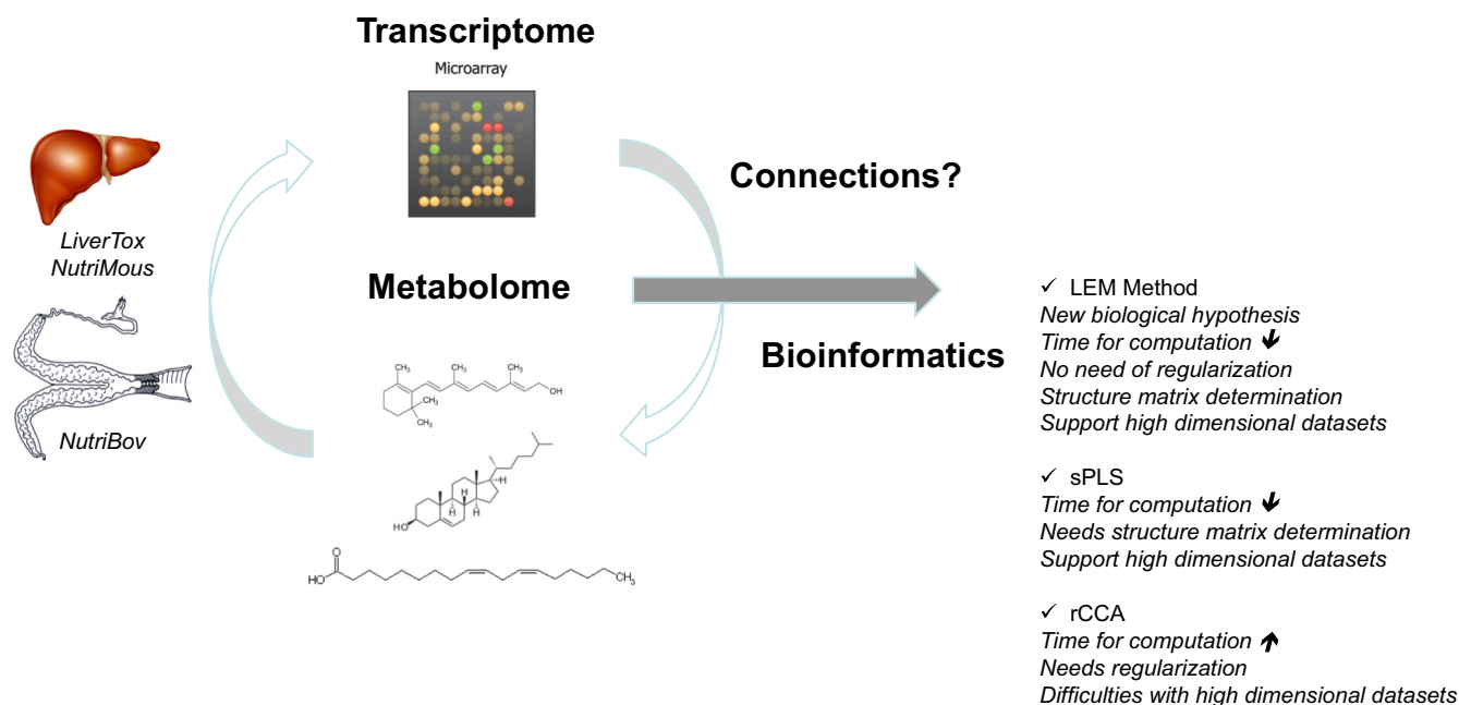
Fig. 9. Summary of the biological questions and the advantages and limits of the LEM method, the sPLS, and the regularized CCA (RCCA).
