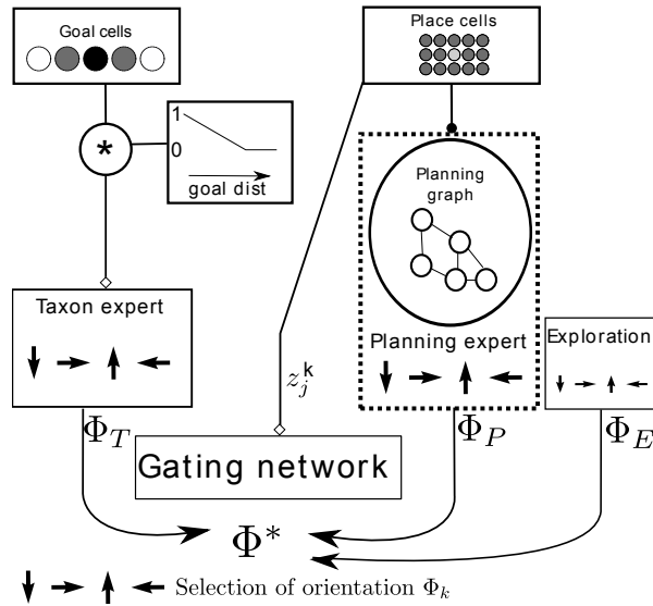
Figure 9. Overview of the gating network with taxon, topological map and exploration experts.
