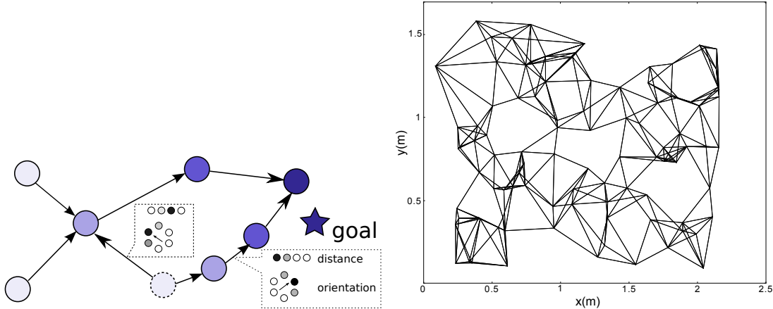
(a) Principle of the topological map. The large circles are the nodes in the map. The goal is on the right and the color of the nodes corresponds to the diffusion values. Direction transition neurons (small circular pattern) and distance transition neurons (4 small circles) are shown for two connections. A path planned from the dashed node can be ambiguous for one node due to equal diffusion values. The robot chooses a next node arbitrarily in this case.
