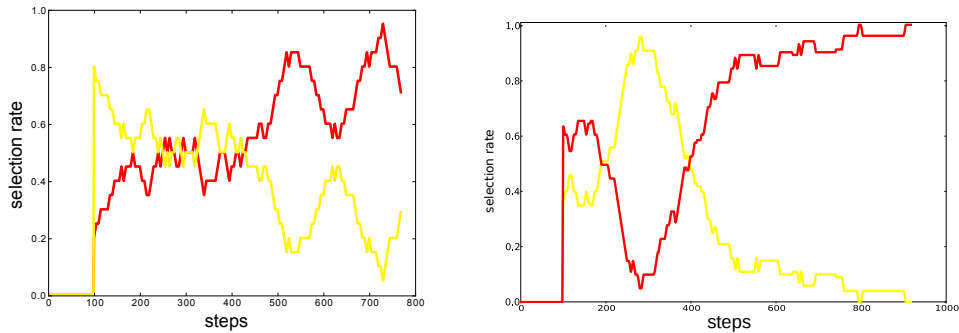
(a) Less precise topological map, resulting in an overall higher selection rate of the planning strategy (b) Very precise topological map, the exploration strategy has very good performance
