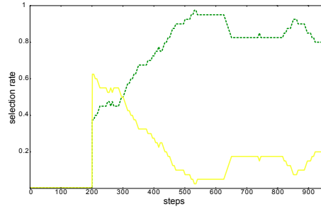
Figure 14. Selection rate of the taxon (dashed dark line) vs. exploration strategy (light line) computed over the last 200 actions. The gating network clearly learned to privilege the taxon strategy.
