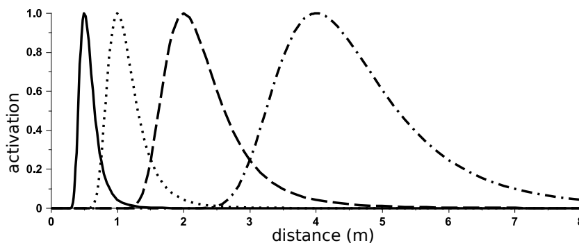
Figure 6. Activation function of the disparity neurons as a function of the distance. They are Gaussian as a function of the disparity, naturally resulting in a non-linear distance scale with higher precision for nearby objects.
