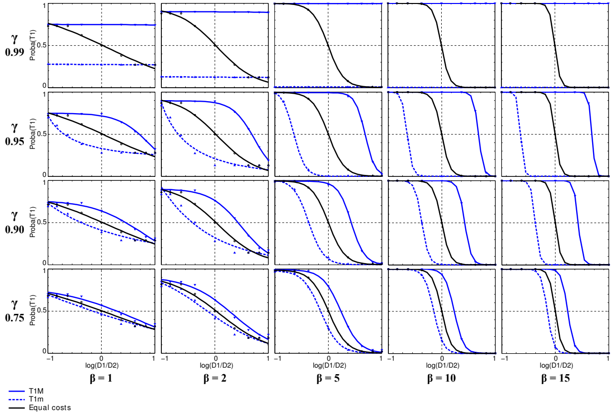
Figure 5: Decisions made by the model during the dynamic programming phase for different parameters \beta and \gamma . For the same transition and reward functions learnt during the motor babbling phase, different parameters in the model can produce different profiles of decisions during the task. As in previous figures, each plot shows the probability of choosing target T1 (as read from the output of the softmax function in equation 5) as a function of the relative distance between the two targets. Increasing \beta produces more steepness in the function and thus a more bistable shift between choosing target T1 and target T2 . Decreasing \gamma flattens the function and reduces the effect of biomechanics in decisions. Increasing \gamma until 0.99 suppresses the influence of relative distance in the choice probability for T1M and T1m cases. The curves shown in figure 4B and illustrating simulations of the model to reproduce the global average effect of biomechanics on decisions were obtained with \beta = 5 and \gamma = 0.90 .
