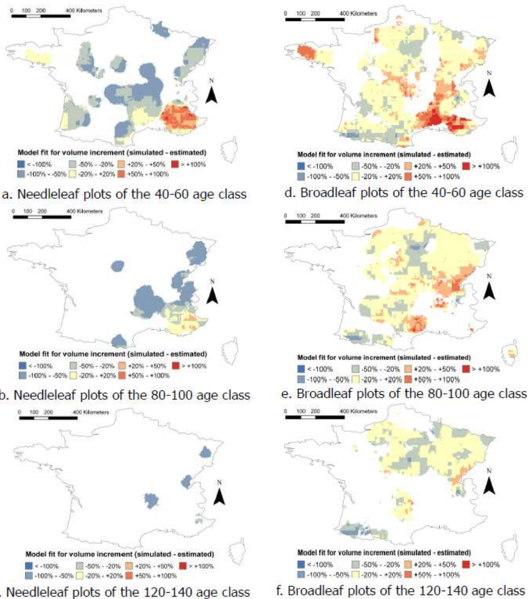
Figure 9. Model fit for the volume increment: evolution with age
