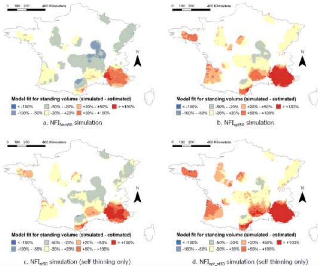
Figure 11. Model fit for standing volume of 50-year-old needleleaf stands
