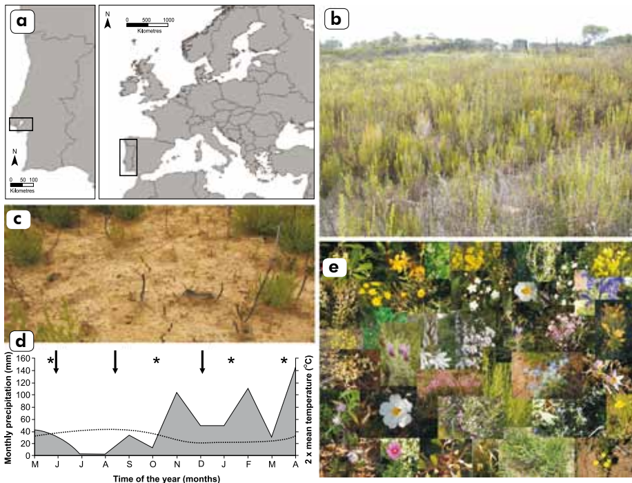
Figure 5.16: a) General location of the studied site; b) landscape view; c) surface soil view; d) mean monthly temperature (dotted line), total monthly precipitation (grey) and times of N additions (arrows) and soil sampling (*) from Spring 2007 to Spring 2008; and e) examples of some of the existing plant species at the study site.
