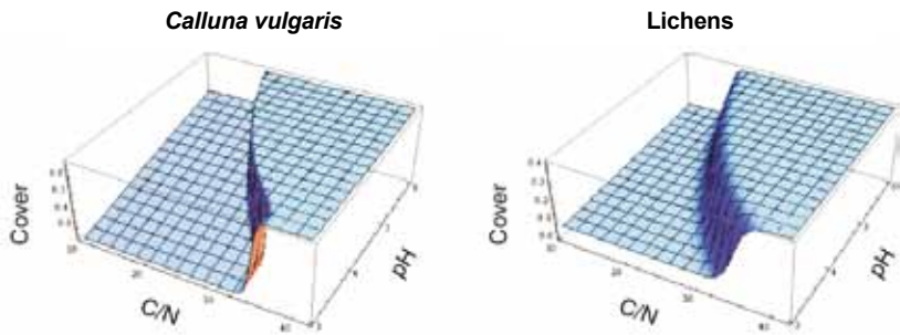
Figure 4.5: Effect of pH and C/N on cover of Calluna vulgaris and lichens on dry dune heathland. The majority of data are around pH 4. The favourable conservation status for C:N ratio in the organic topsoil is > 30 which is clearly seen as a threshold
