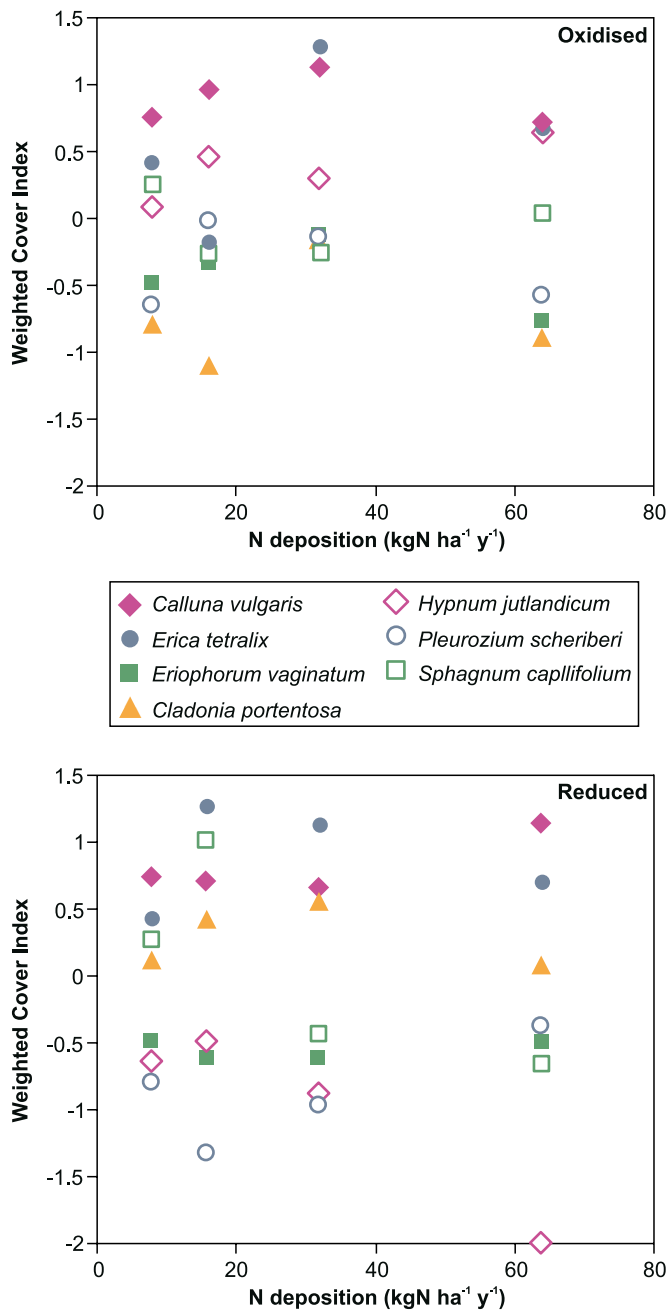
Figure 5.25: Change in the weighted cover index (value based on start value and after five years exposure) for vascular and non vascular plants treated with wet oxidised and wet reduced nitrogen as \text{NaNO}_3 or \text{NH}_4\text{Cl} , respectively. The species represented are the most common species growing at the experimental site an ombrotrophic bog, Whim in Southern Scotland. Values above the bold line represent an increase in cover and vice versa. Cover at 8 \text{ kg N ha}^{-1} \text{y}^{-1} represents the control response, receiving no additional N.
