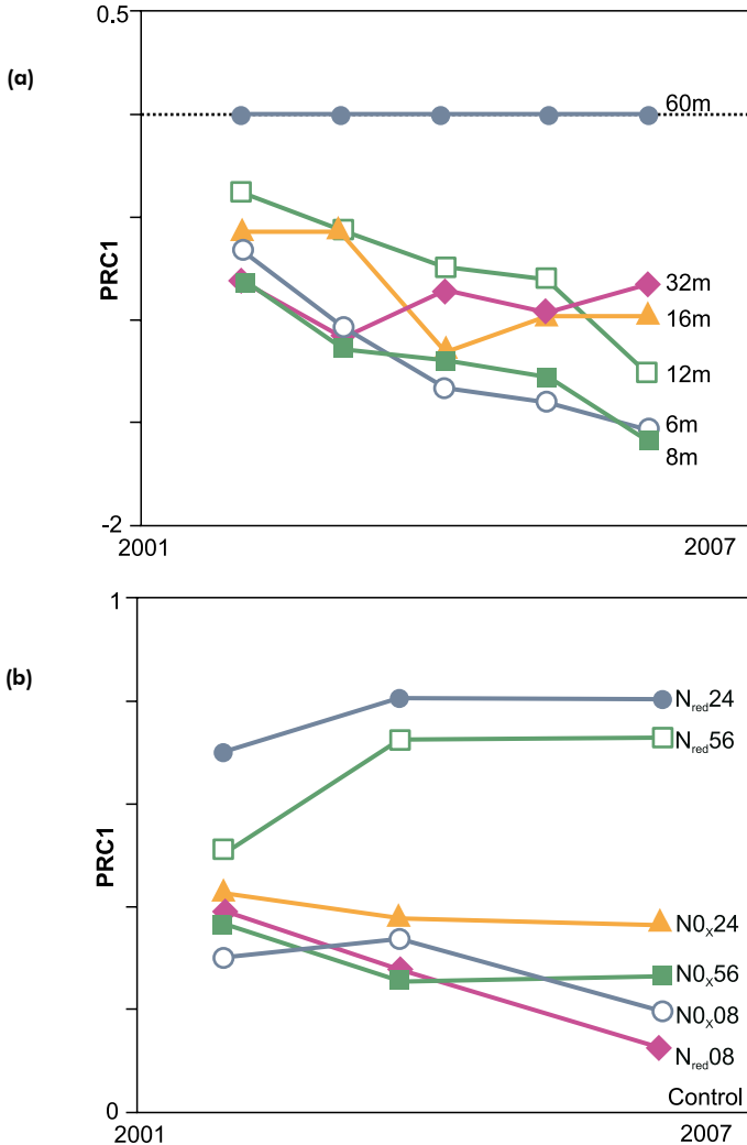
Figure 5.26: Principal Response Curves (PRC) based on redundancy analysis (RDA) of the vegetation cover data from dry and wet N deposition treatments at Whim Moss. (a) PRC for dry N treatment vegetation. (b) PRC for wet N treatment vegetation. The curves represent the temporal trajectory of community composition for each of the experimental treatments
