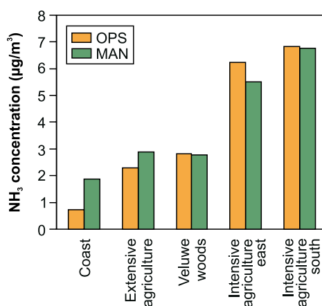
Figure 6.2: Operational Priority Substances (OPS) model and Measuring Ammonia in Nature (MAN) monitoring network values for ammonia concentration ( \mu\text{g m}^{-3} ), averaged over a number of Natura 2000 areas in the South and East of the Netherlands.
