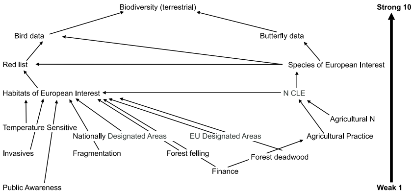
Figure 5.12: Linkages between the terrestrial SEBI 2010 indicators and their relationship with biodiversity
