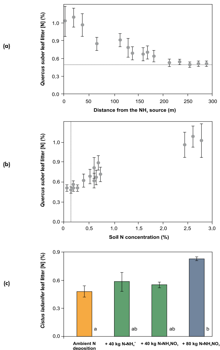
Figure 7.12a,b,c: Changes in leaf litter N concentration in response to increased N availability in two Natura 2000 sites in Portugal that correspond to different Mediterranean-type ecosystems: a) relation between leaf litter N (mainly Quercus suber leaves – collected in the four seasons in 2008) concentration and distance to a source point of ammonia (barn with 200 cows, Pinho et al. , 2009) in a cork oak system (values represent mean \pm sd; n = 4 sampling points); b) relation between leaf litter N concentration (collected in summer 2008), and soil N concentration in the same cork oak system as in a); c) relation between leaf litter N concentration from Cistus ladanifer and N additions beginning in 2007 in a semi-natural Mediterranean Maquis (bars represent mean values \pm se; N = 3 experimental plots per treatment).
