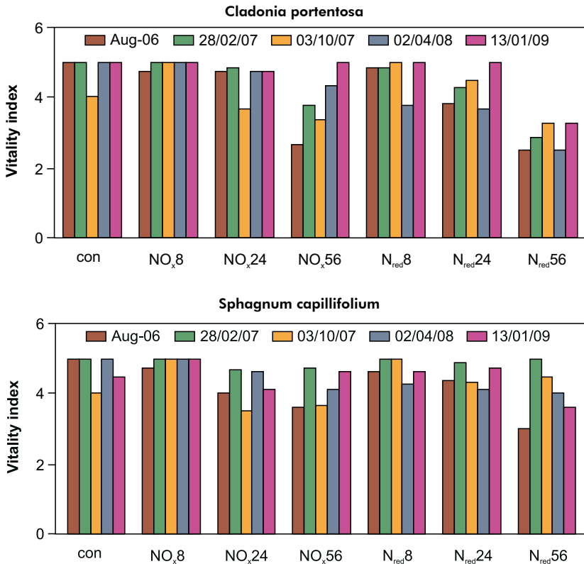
Figure 5.19: Vitality Indices, subjective scoring of visible damage where a maximum score of five constitutes healthy, for Cladonia portentosa and Sphagnum capillifolium treated with sodium nitrate (NO x ) or ammonium chloride (Nred) in rainfall at 8, 24 or 56 kg N ha -1 y -1
