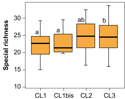
Figure 5.9: Box plots showing species richness (mean SR.m -2 ; n=5 replicates) variations in the four clusters from the CA. see text for details. Boxes sharing the same letter are not statistically different (P < 0.05, Tukey's HSD comparing all clusters).
