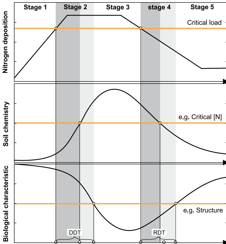
Figure 4.2: Possible stages of influence of N-deposition on conservation status. Adapted from CCE 1 [DDT = Damage Delay Time, RDT = Recovery Delay Time]
