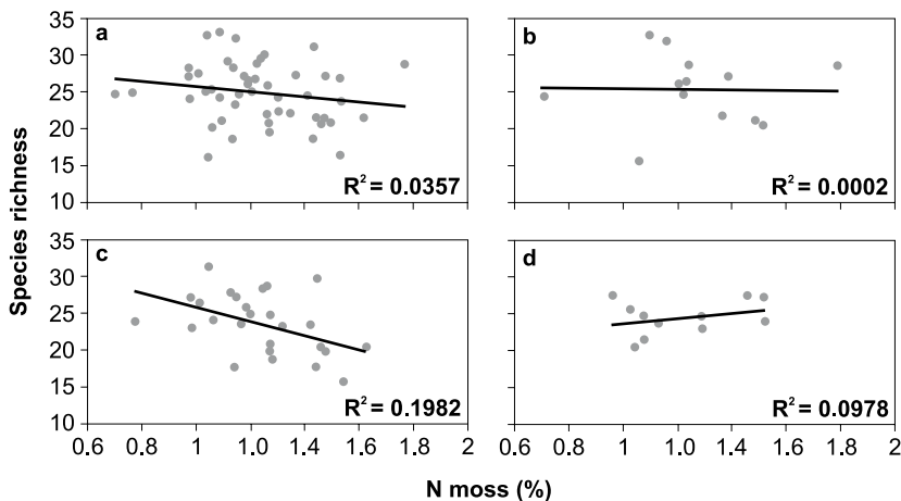
Figure 5.10: Regression plots between nitrogen concentration in the moss Ctenidium molluscum (N per cent dry weight) and species richness (mean SR.m -2 ; n=5 replicates) in calcareous grasslands according to different geographic ranges: a) subset covering the whole geographic range i.e. Atlantic Europe; n=51 ; b) subset from NW Atlantic Europe i.e. Cluster 3; c) subset from SW Atlantic Europe i.e. Cluster 2; subset from Eastern Atlantic Europe i.e. Cluster 1. See text for details.
