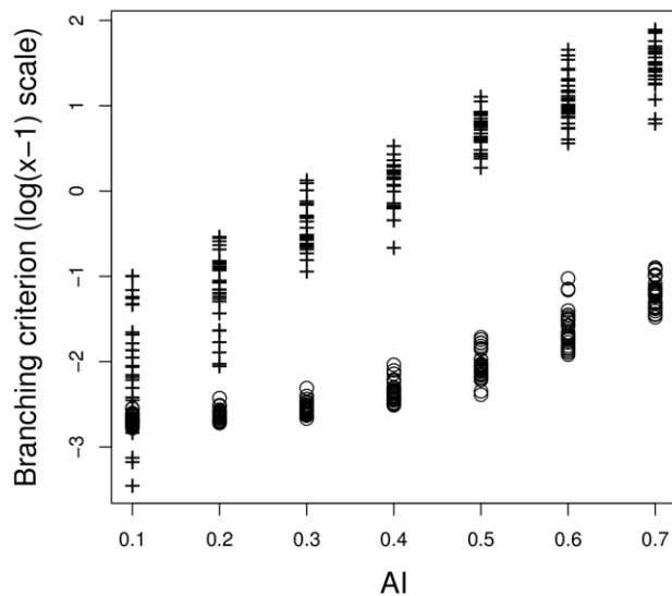
Figure 4. Value of the branching criterion against the aggregation index (AI). Open circles, situation A ( m_s=75\% , \delta/\sigma=1.1 ( \delta = -\beta_1 = \beta_2 = 1.1 and \sigma=1 ) and \pi=0.32 ); pluses, situation B ( m_s=15\% , \delta/\sigma=1.1 ( \delta = -\beta_1 = \beta_2 = 1.1 and \sigma=1 ) and \pi=0.16 ). The lattice environment was used. doi:10.1371/journal.pone.0054697.g004
