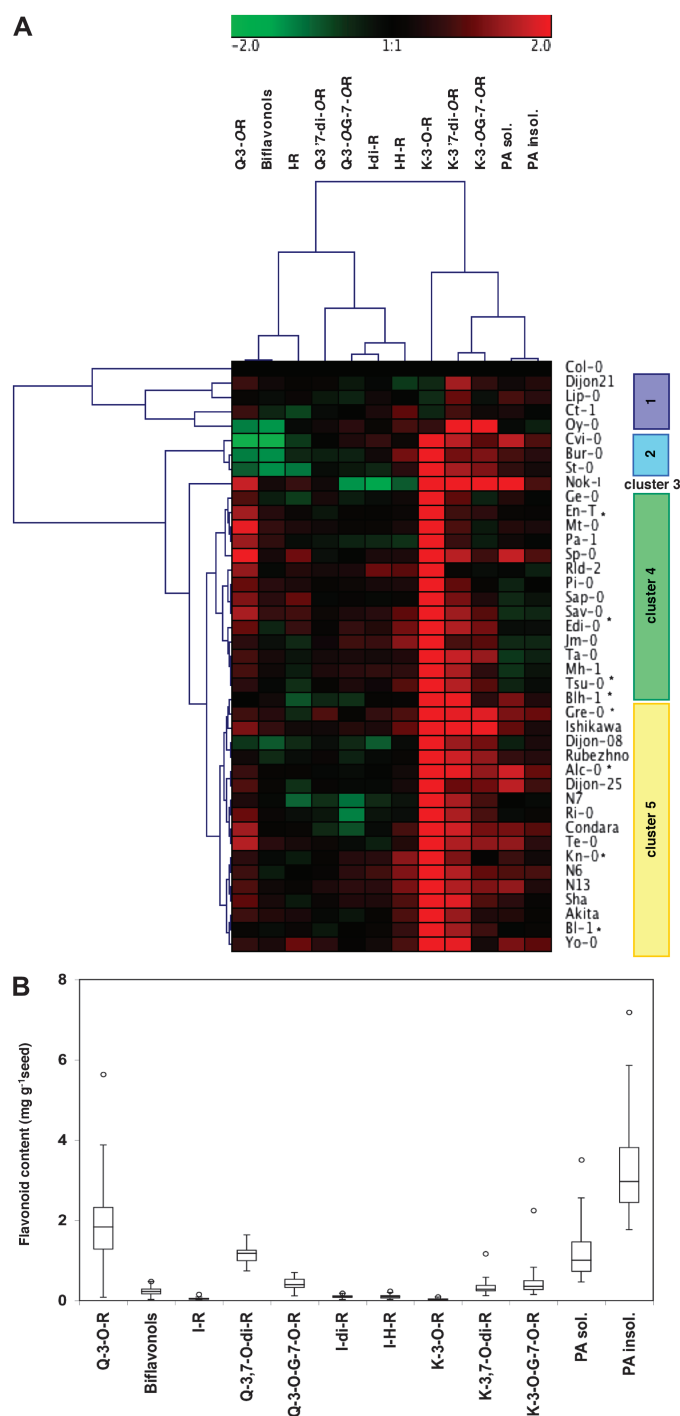
Fig. 2. Natural variation of seed flavonoids in Arabidopsis . (A) Hierarchical clustering analysis of mature seed flavonoid accumulation in 40 accessions compared with Col-0. Log2 % of from three (*or two) independent measurements \pm SE. Flavonoid contents for each accession and correlation between the different compounds are given in Supplementary Tables S1 and S2, respectively, at JXB online. (B) Boxplot analysis of flavonoid content in accessions giving the minimum, lower quartile, median, upper quartile and outlier, respectively, from bottom to top. G, glucoside; H, hexoside; I, isorhamnetin; insol., insoluble; K, kaempferol; Q, quercetin; PA, proanthocyanidin; R, rhamnoside; sol., soluble.
