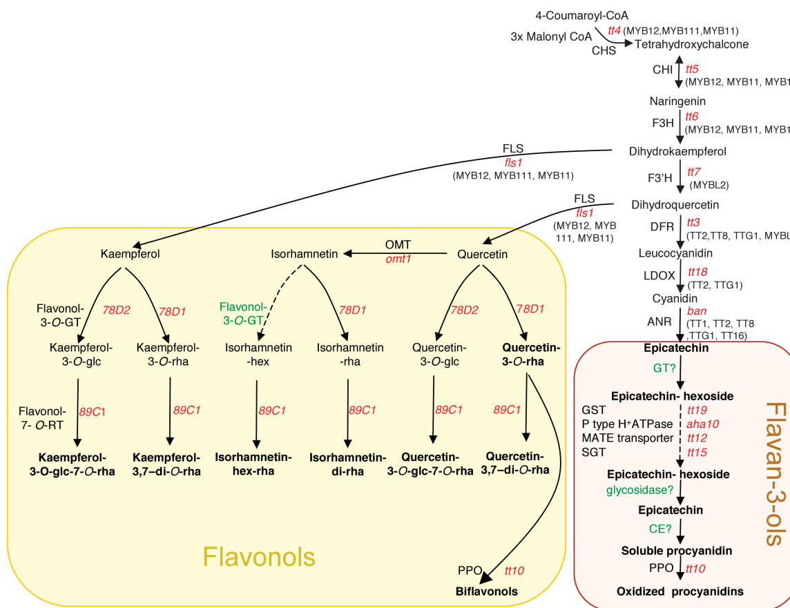
Fig. 1. The flavonoid biosynthetic pathway in Arabidopsis seed. The different steps leading to the formation of flavonoids in Arabidopsis seed are indicated by arrows. Major flavonoids are indicated in bold. Mutants for enzymatic steps are indicated in red lower case italic letters. Regulatory proteins are given in parentheses beside their target genes that are shown in upper case letters. ANR, anthocyanidin reductase; ANS, anthocyanidin synthase (LDOX, leucoanthocyanidin dioxygenase); CE, condensing enzyme; CHI, chalcone isomerase; CHS, chalcone synthase; DFR, dihydroflavonol-4-reductase; F3H, flavonol 3-hydroxylase, F3'H, flavonoid 3'-hydroxylase, FLS, flavonol synthase; glc, glucose; GST, glutathione S-transferase; GT, glycosyltransferase; hex, hexose; OMT, methyltransferase; PPO, polyphenol oxidase; rha, rhamnose; RT, rhamnosyltransferase; SGT, UDPglucose:sterol glucosyltransferase. Steps that still need to be characterized are indicated in green with a question mark.
