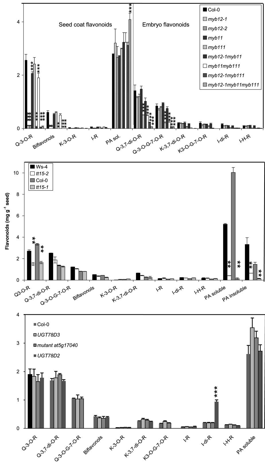
Fig. 6. Flavonoid analysis of mutants for genes located near the FLA loci. G, glucoside; H, hexoside; I, isorhamnetin; K, kaempferol; Q, quercetin; PA, proanthocyanidin; R, rhamnoside; sol., soluble. Significance in t -test compared with the wild type at the *5%, **1%, and ***0.1% level.
