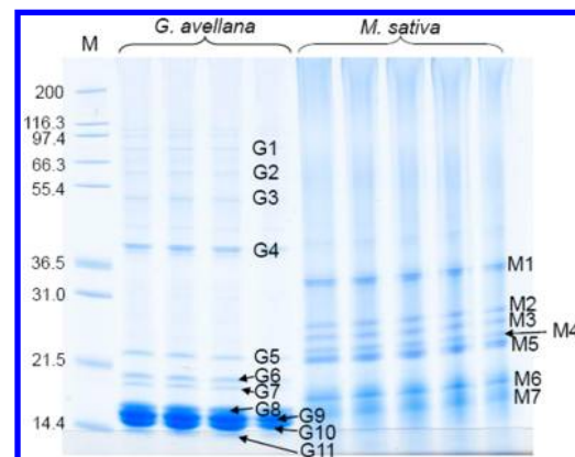
Figure 4. SDS-PAGE of proteins from isolated oil bodies from G. avellana and M. sativa seeds (10 \mu g protein/lane). Molecular mass marker (M) was Mark 12 from Novex. Coomassie-blue stained protein bands were numbered as listed in Tables 3 and 4 and in the Supporting Information.
