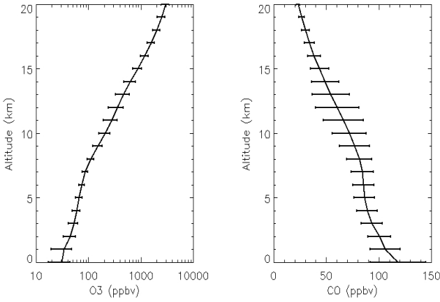
Fig. 1. MOCAGE O 3 and CO a priori profiles and variances (diagonal elements of \mathbf{S}_e ) considered in this study.
