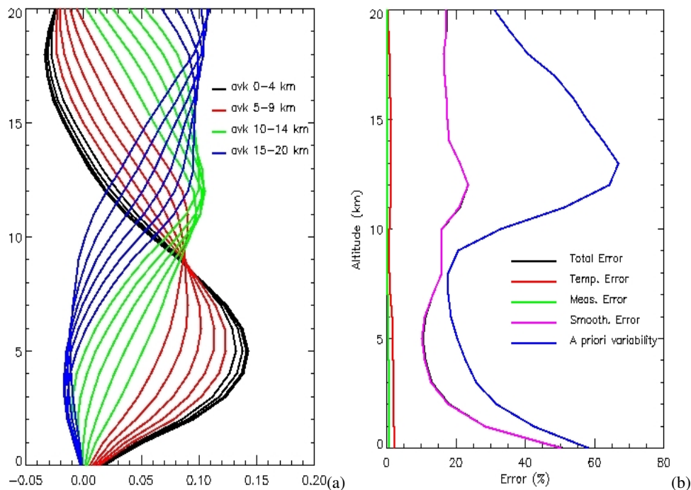
Fig. 4. (a) Averaging kernels obtained for the O 3 retrieval for a thermal contrast of 0 K: spectral sampling interval of 0.05 and a Signal to Noise Ratio (SNR) of 750 (0–4 km: black, 5–9 km: red, 10–14 km: green, 15–20 km blue); (b) error budget as a function of altitude for different error sources (see legend) for the same instrument characteristics as in part (a).
