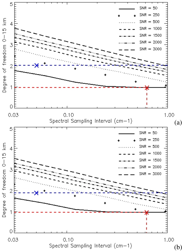
Fig. 3. Same as Fig. 2 but for CO.
