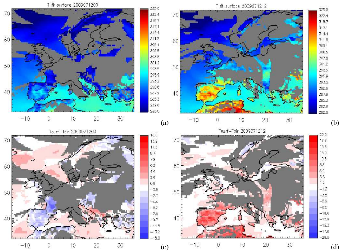
Fig. 7. Surface temperature in K (a, b) and thermal contrast (surface temperature minus air temperature near the surface) in K (c, d) on 12 July 2009 from ARPEGE: (left) 00:00 UTC; (right) 12:00 UTC. Grey areas represent pixels with more than 50% of cloud fraction. In (c, d) red indicates surface temperature is higher than the air temperature; blue indicates surface temperature is lower than the air temperature.
