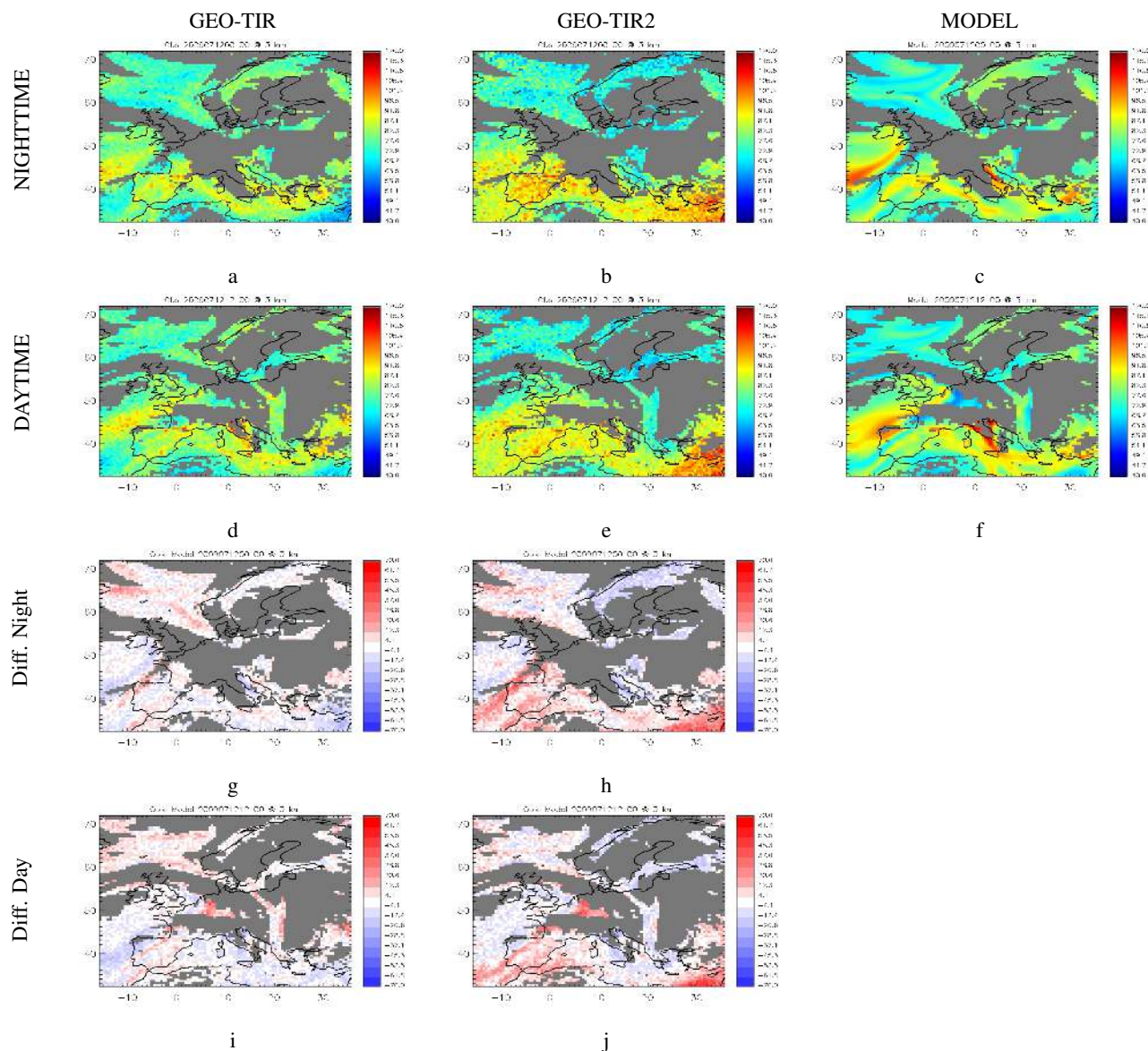
Fig. 10. Same as Fig. 8 but for CO.
