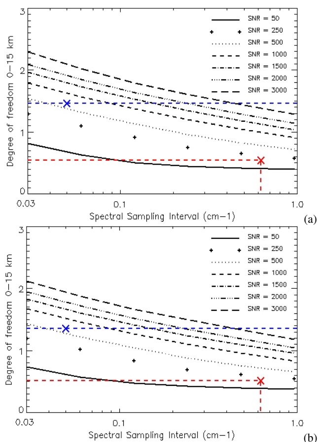
Fig. 2. Degrees of freedom (DOF) obtained for the O 3 retrieval as a function of spectral sampling interval and instrument noise (SNR): (a) positive thermal contrast (+2 K); (b) negative thermal contrast (−2 K). The DOFs have been obtained for an idealized case where all the parameters (e.g., regularization) are fixed except the SNR and the spectral resolution. The reference profile used to generate the synthetic measurement spectral radiances and representing the true profile in the retrieval study is an average of MOCAGE O 3 over Europe from 1 July 2009 to 31 August 2009 during daytime for the positive thermal contrast and during nighttime for the negative thermal contrast. The SNR is calculated for a surface temperature of 280 K. The blue cross corresponds to the GEO-TIR instrument configuration and the red cross corresponds to GEO-TIR2 instrument configuration.
