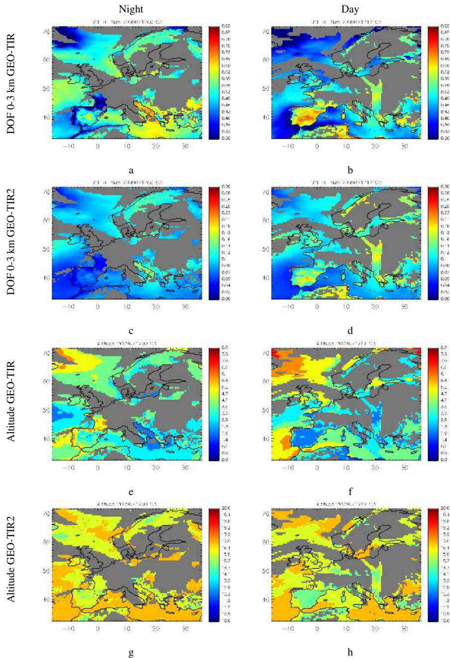
Fig. 9. Degrees of Freedom obtained for O 3 with GEO-TIR (a, b) and with GEO-TIR2 (c, d) instrument configuration on 12 July 2009 at 00:00 h UTC (left) and at 12:00 h UTC (right). The peak altitude (km) of the lowermost averaging kernels are represented for GEO-TIR (e, f) and for GEO-TIR2 (g, h) on 12 July 2009 at 00:00 h UTC (left) and at 12:00 h UTC (right). Grey areas represent pixels with more than 50% of cloud fraction. Note that the colour scales are different for GEO-TIR and GEO-TIR2.
