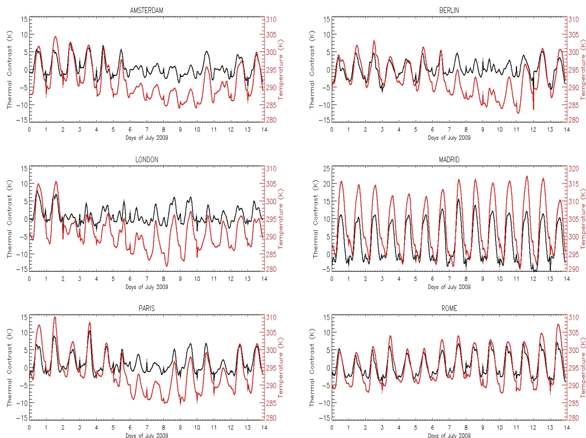
Fig. 13. Time-series of temperature at surface (red) and thermal contrast (black) in K from ARPEGE model from 1 July 2009 to 15 July 2009 with a temporal resolution of 1 h over 6 European cities: Amsterdam, Berlin, London, Madrid, Paris and Rome.
