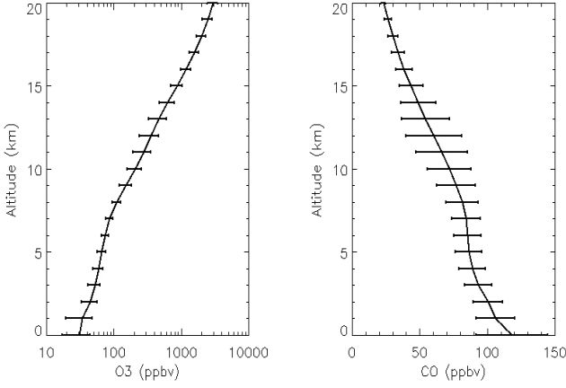
Fig. 1. MOCAGE O 3 and CO a priori profiles and variances (diagonal elements of \mathbf{S}_e ) considered in this study.
