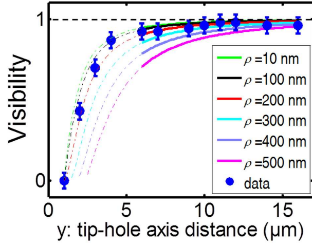
Figure 3. Visibility as a function of tip-hole axis distance ( y ): the blue dots show the data obtained from figures such as figure 2(b)-(i) above. The curves are obtained from equations 7 and 8 with d = 2 \mu\text{m} and \lambda_0 = 700 \text{ nm} ; \rho is the radius of the source. Note that equation 8 is only valid for y \gg d , i.e., for tip-hole axis distances that are large as compared to the hole separation.
