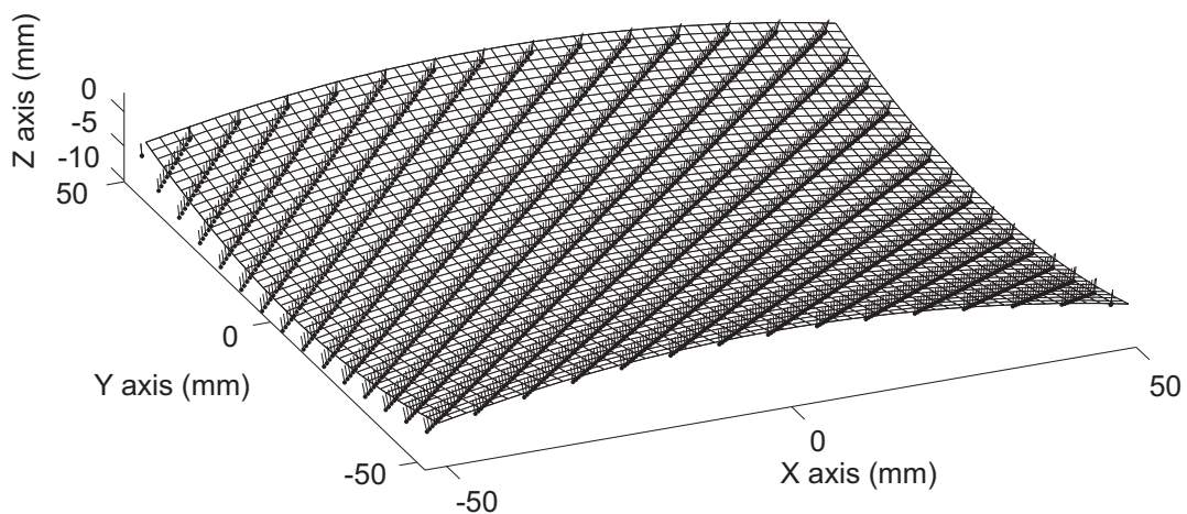
Figure 4; Calculated tool-path
