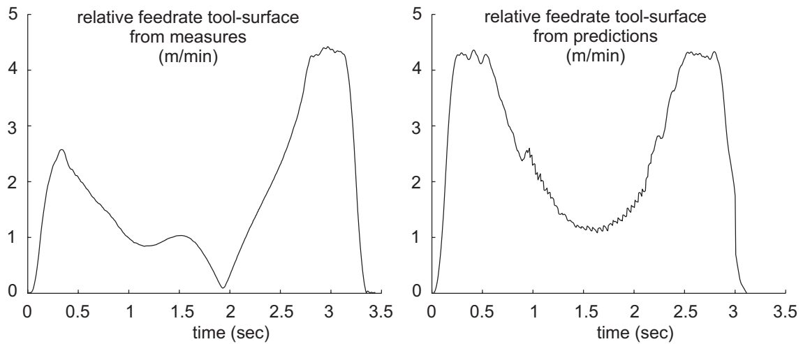
Figure 6; Comparison between measured and predicted relative feed rate
