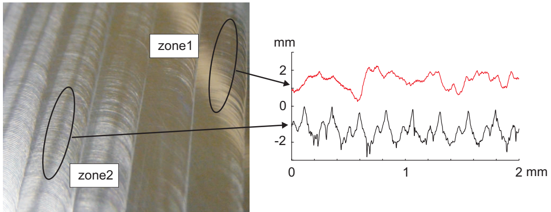
Figure 7; Comparison of the tooth track according zones
