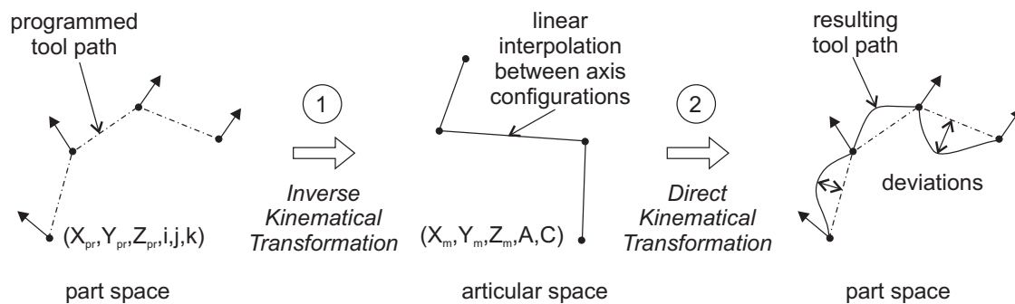
Figure 2; Influence of the linear interpolation in the joint space on the tool path.
