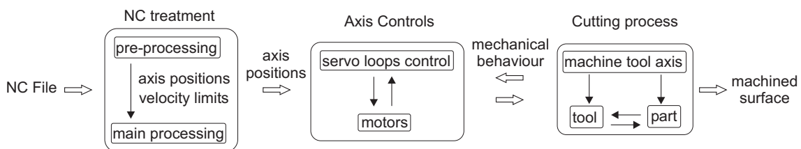
Figure 1; NC file treatment to machined surface
