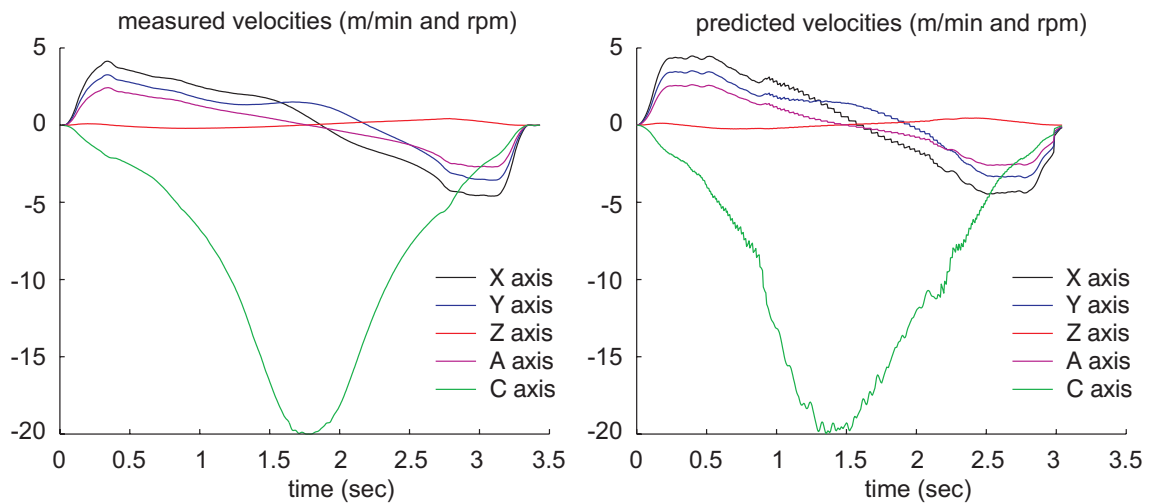
Figure 5; Comparison between measured and predicted axis velocities
