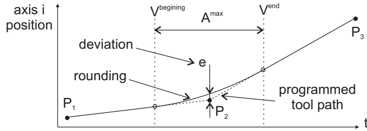
Figure 3; Rounding tangency discontinuity.
