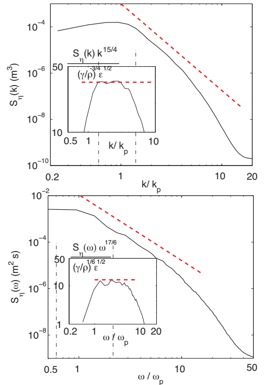
FIG. 3. (a): S_\eta(k/k_p) . (b): S_\eta(\omega/\omega_p) . Theoretical KZ spectrum (---) is respectively S_\eta \sim k^{-15/4} and S_\eta \sim \omega^{-17/6} . Inset: compensated spectrum, respectively S_\eta(k)k^{15/4}/(\epsilon^{1/2}(\gamma/\rho)^{-3/4}) and S_\eta(\omega)\omega^{17/6}/(\epsilon^{1/2}(\gamma/\rho)^{1/6}) . Vertical dot-dashed line indicates the forcing scale range.
