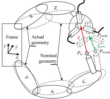
Fig. 1: Schematic view of the volumetric error
