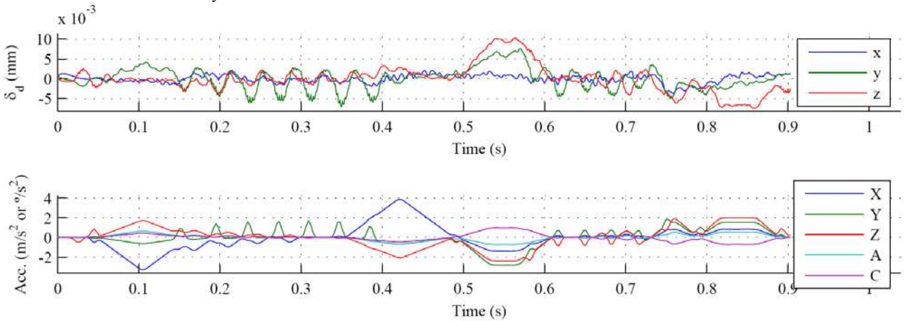
Fig. 3: Evolution of \delta_d and acceleration for a programmed feed rate F = 18\,896\text{ mm/min}
