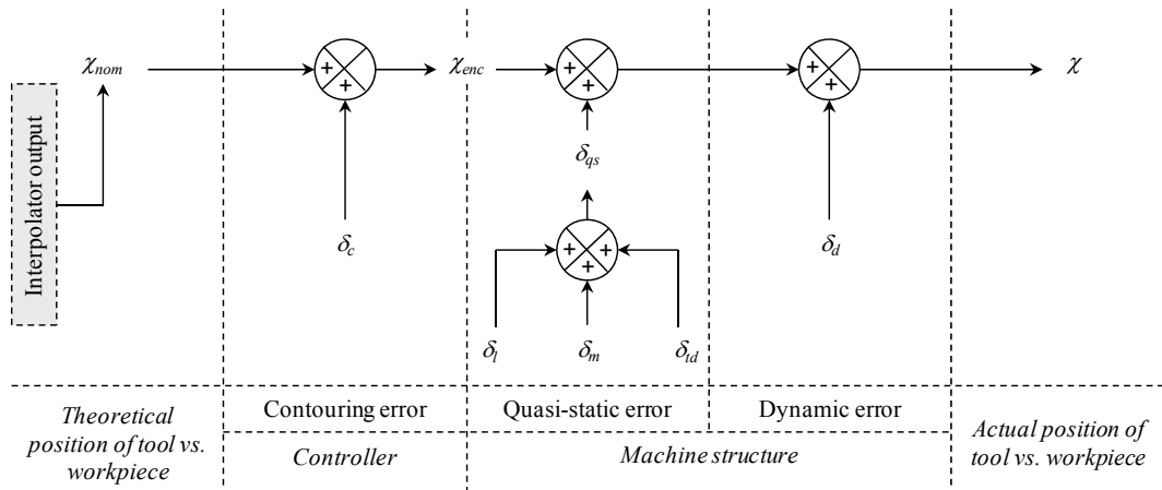
Fig. 2: Decomposition of the error into contouring error \delta_c , quasi-static geometric error \delta_{qs} and dynamic geometric error \delta_d .
