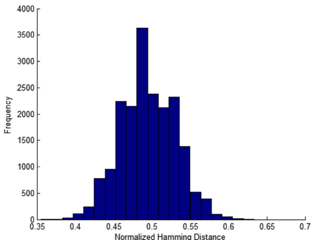
Fig. 7 – Pseudo-impostor distribution histogram.
