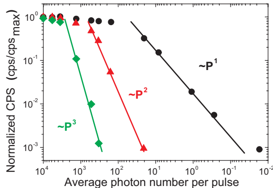
FIG. 3. (Color online) Dependence of normalized counts per second vs incoming light power. Circles (black), triangles (red) and diamond (green) symbols, respectively, correspond respectively to a linear, quadratic ( \propto P^2 ) and cubic ( \propto P^3 ) dependence and thus to single, two, and three-photon regime because the counts per seconds are proportional to P^n , where P is the light power and n the number of photons detected.
