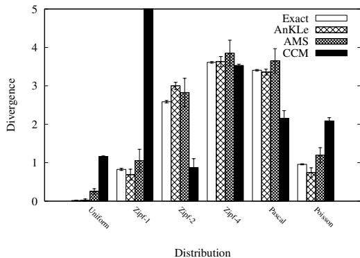
(a) Comparisons between the Uniform distribution and the Uniform, Zipf-1, Zipf-2, Zipf-4, Pascal and Poisson distributions.
