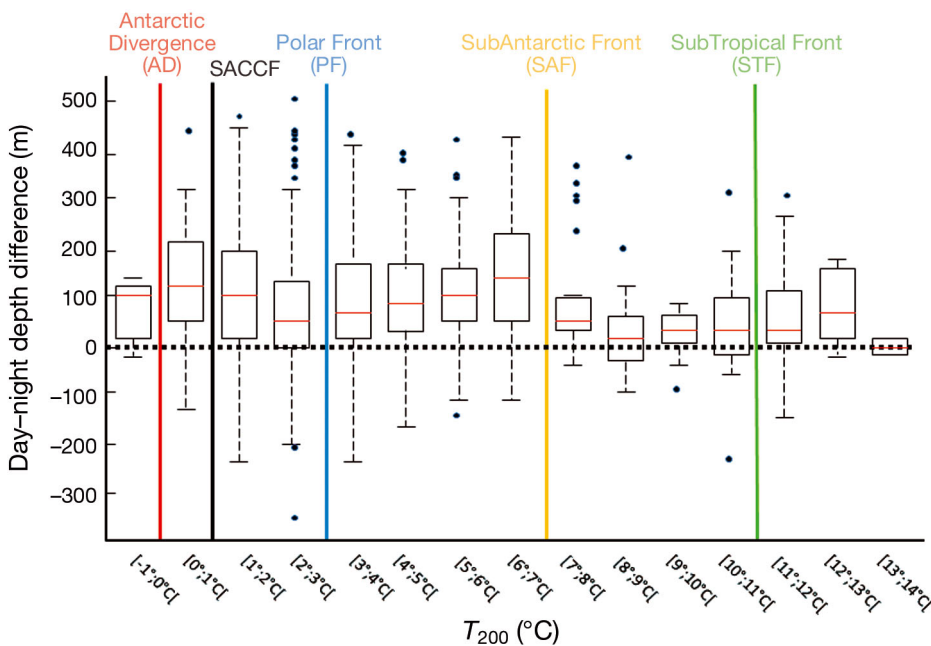
Fig. 4. Box plot of the mean depth differences between day and night dive according to each 1^\circ\text{C} temperature at 200 m ( T_{200} ) class. Horizontal lines represent the median, the box represents the 0.75 to 0.25 quartiles, and whiskers represent 1.5 times the interquartile range (IQR). Small circles represent outliers (i.e. values exceeding 1.5 times IQR). SACC: Southern Antarctic Circumpolar Current Front.
