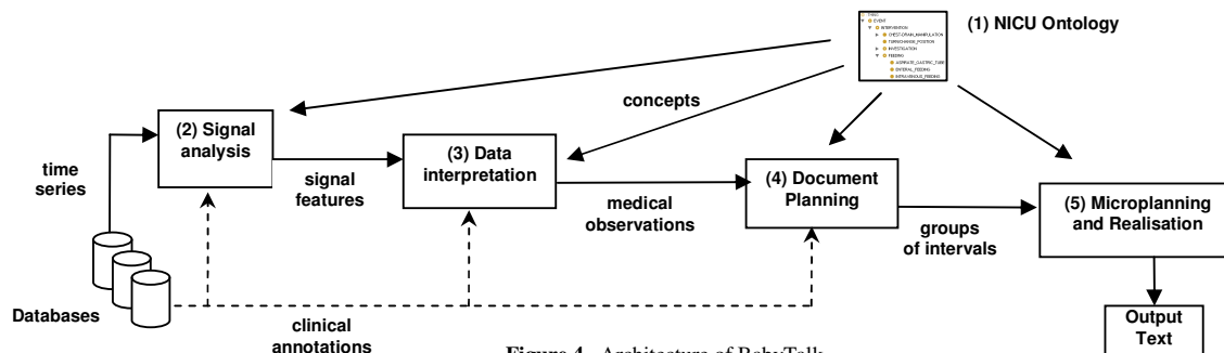
Figure 4. Architecture of BabyTalk
