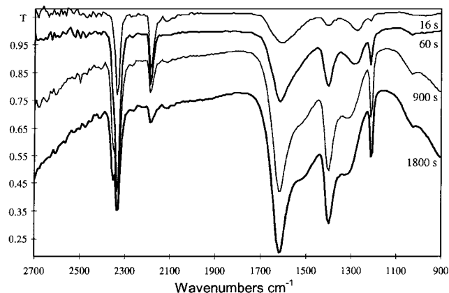
FIG. 10. Changes with time of spectra recorded on outgassed \text{NiMn}_2\text{O}_{4+\delta} under a flowing gas mixture, \text{CO} (2\%) + \text{O}_2 (1\%) + \text{N}_2 (balance), at 253\text{ K} . Spectra are offset for clarity.
