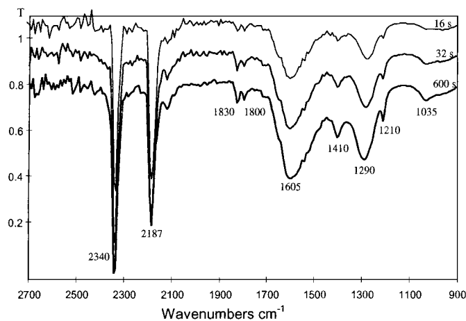
FIG. 8. Changes with time of FTIR spectra recorded on outgassed \text{NiMn}_2\text{O}_{3\delta/4}\text{O}_{4+\delta} under \text{CO} ( 10^3 Pa) at 253 K. Spectra are offset for clarity.
