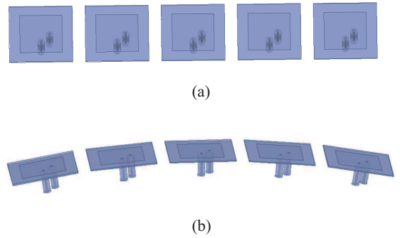
Fig. 1. Geometry of the array composed of five dual polarized patches: (a) top view of the linear array and (b) side view of the conformal array.
