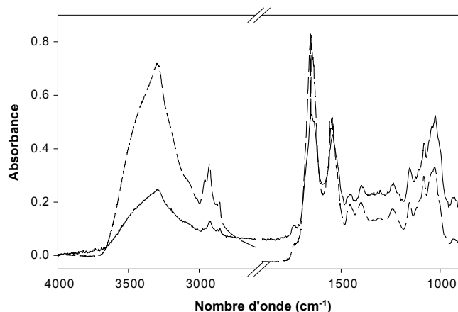
Fig. 3 Comparison between the mouse liver spectra recorded in transmission mode (solid line) and with the optical fiber (dashed line). 42
