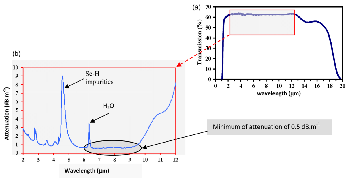
Fig. 1 (a) Transmission window for a bulk of \text{Te}_2\text{As}_3\text{Se}_5 glass (thickness 1 mm) together with the attenuation curve of the TAS glass fiber (b). 40
