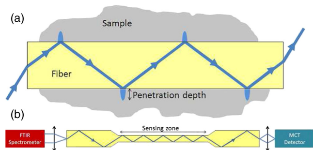
Fig. 2 (a) Mechanism of fiber evanescent wave spectroscopy (FEWS). (b) General setup of FEWS and the scheme of a tapered fiber. 4
