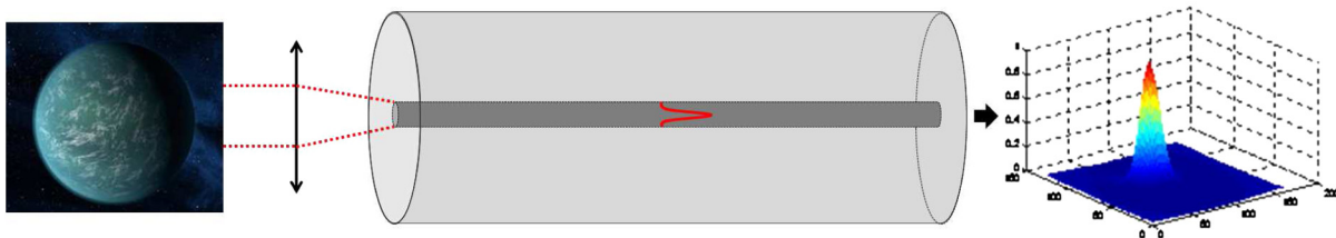
Fig. 7 Optical scheme of the detection of the mid-IR signal coming from an exo-planet through space. The beam profile on the right corresponds to a single-mode TAS glass at 10 \mu\text{m} .
