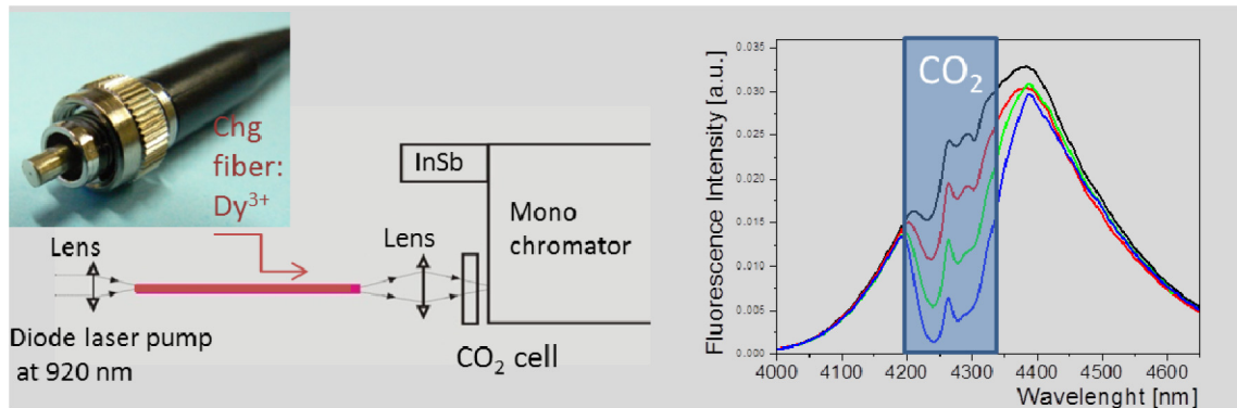
Fig. 6 Fluorescence spectra of \text{Dy}^{3+} -doped chalcogenide glass showing the \text{CO}_2 absorption bands around 4.3 \mu\text{m} pumped by commercial diode laser at 920 \text{ nm} .
