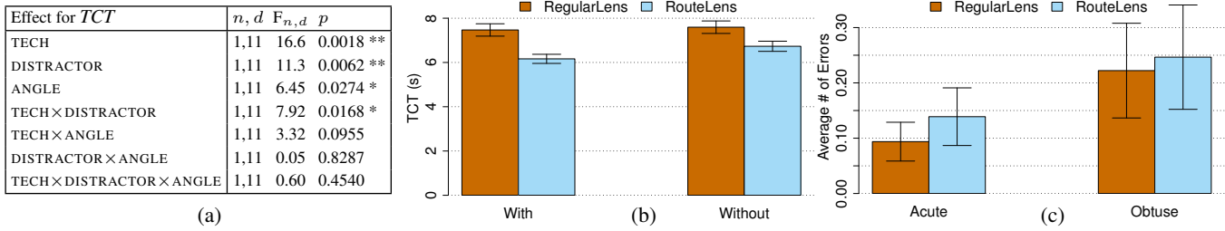
Figure 4: (a) ANOVA for the full factorial model TCT \sim \text{TECH} \times \text{DISTRACTOR} \times \text{ANGLE} \times \text{Rand}(\text{PARTICIPANT}) . (b) TCT by \text{TECH} \times \text{DISTRACTOR} condition. (c) Average number of errors by trial, by \text{TECH} \times \text{ANGLE} condition. Error bars show the confidence interval for the mean over all trials.
