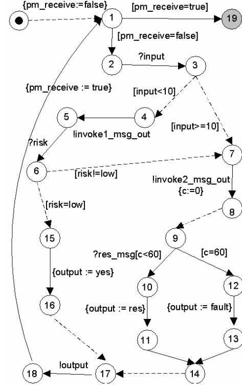
Figure 8. TEFM of the Loan Web Service
