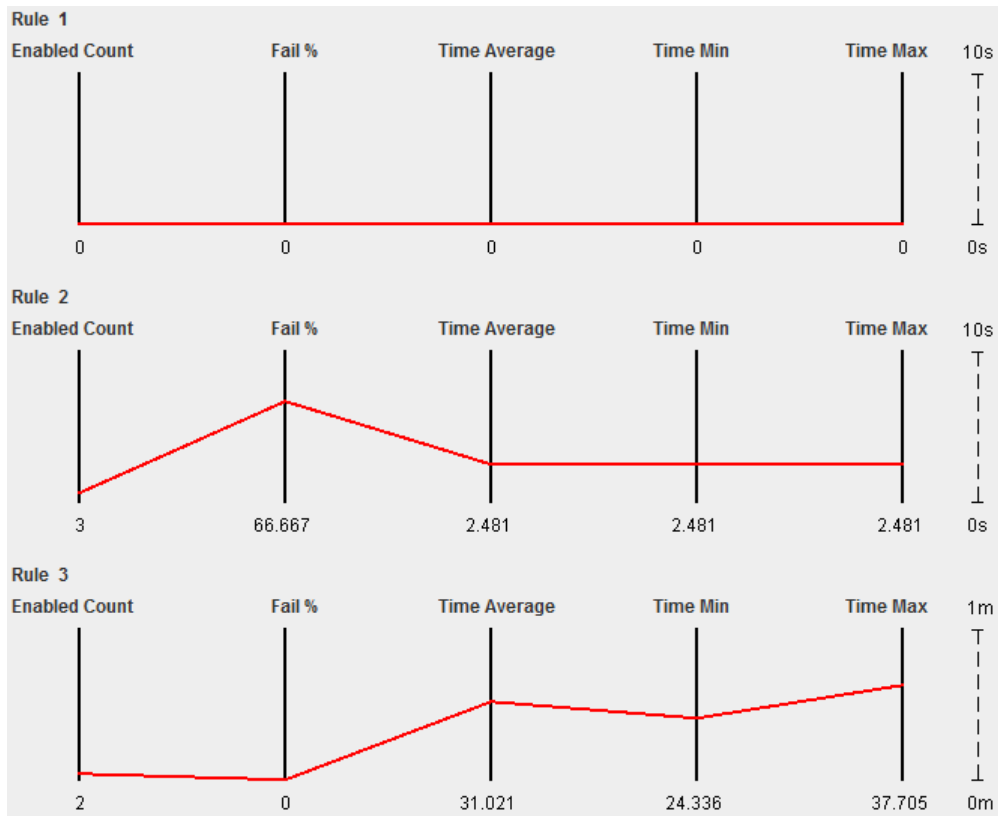
Fig. 8. Checking analysis of Product Retriever
