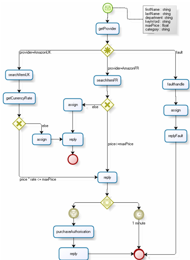
Fig. 6. ProductRetriever - BPMN specification
