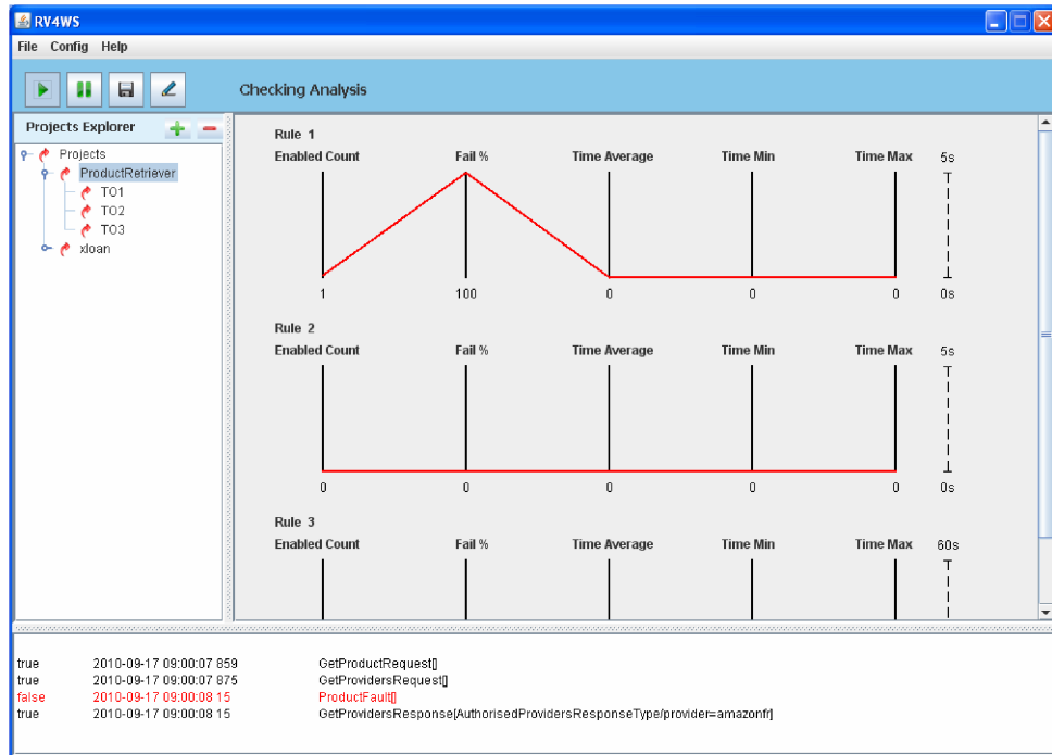
Fig. 5. The main GUI and checking analysis of RV4WS tool
