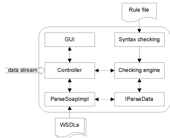
Fig. 2. Architecture of the RV4WS tool
