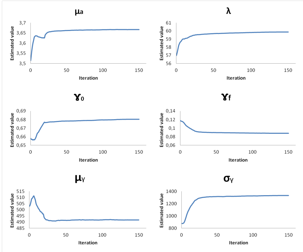
Figure 1: Evolution of the estimated values of six functional parameters: \mu_a , \lambda , \gamma_0 , \gamma_f , \mu_\gamma and \sigma_\gamma with the RPF-EM algorithm (150000 particles) for the restricted dataset.
