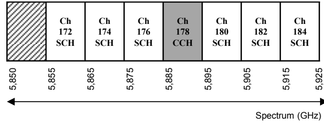
Figure 5: DSRC band plan channel designations
