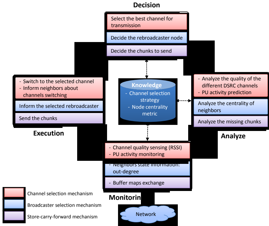
Figure 4: ViCoV architecture
