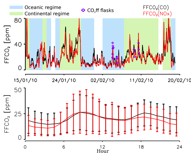
Fig. 7. Top: time series for FFCO 2 during the MEGAPOLI campaign calibrated using CO and NO x as proxies. The purple rhombuses correspond to the CO 2ff from the flasks sampling. Periods during which the air masses originate from the west are highlighted in blue, and periods during which the air masses originate from the east are highlighted in green. No colour is attributed on the days without a clear air mass origin (see Fig. 2). Bottom: mean diurnal cycles of FFCO 2 (CO) in black and FFCO 2 (NO x ) in red at the LHVP station from 15 January 2010 to 19 February 2010.
