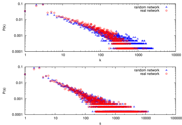
Figure 2. Real (red circles) and random (blue triangles) epistemic network distributions of degrees (up) and strengths (bottom)
