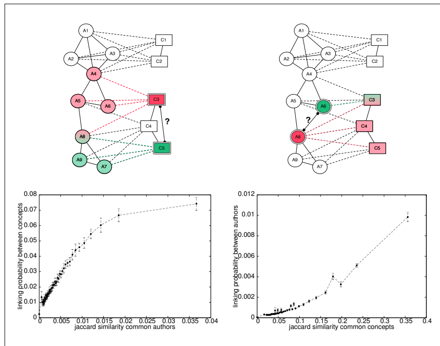
Figure 6. (Left) Linking probability between two concepts in the epistemic network in function of common authors Jaccard similarity. (Right) Linking probability between two authors in the social network in function of common concepts Jaccard similarity. Values are averaged over all the considered years, and the error bars represent the 95% confidence level interval.
