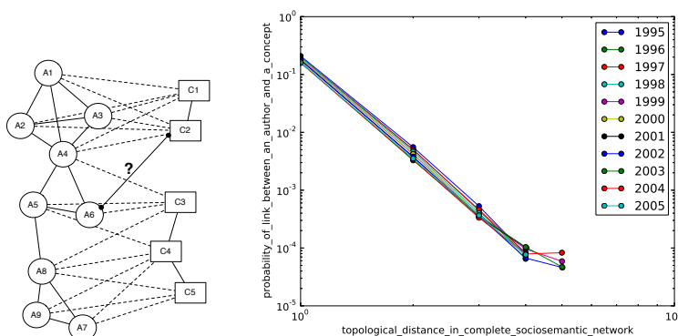
Figure 7. (Left) Linking probability that an author (here A6) will use a given concept (here C2) in function of topological distance computed in the common authors Jaccard similarity. The probability for an author to use a concept is exponentially decreasing with their topological distance in the hybrid socio-epistemic network.
