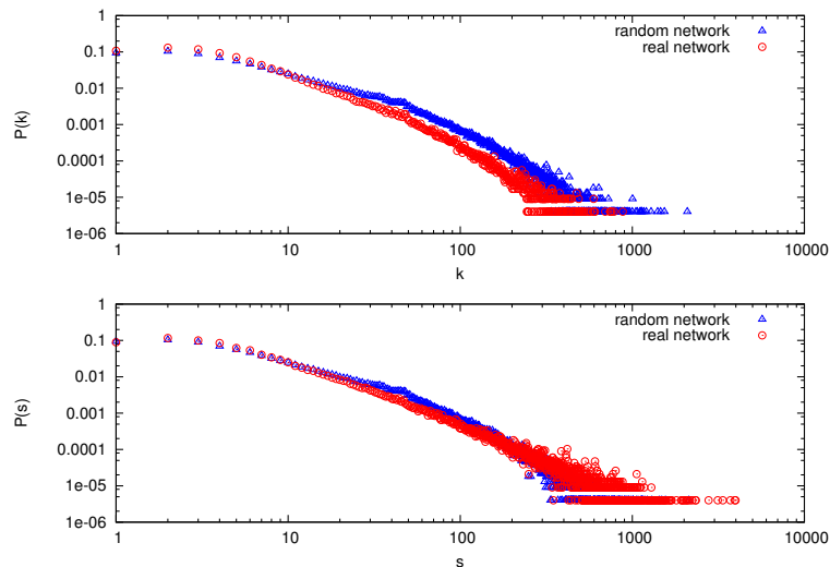
Figure 3. Real (red circles) and random (blue triangles) social network distributions of degrees (up) and strengths (bottom)
