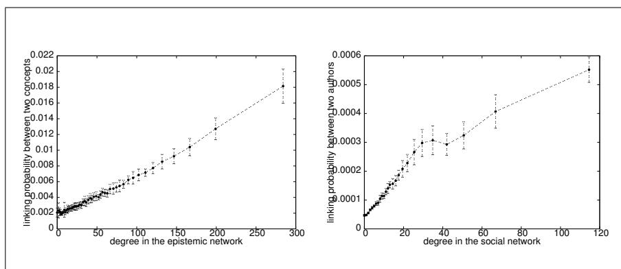
Figure 4. (Left) Linking probability between two concepts in the epistemic network in function of their degree. (Right) Linking probability between two authors in the social network in function of their degree. Values are averaged over all the considered years, and the error bars represent the 95% confidence level interval.
