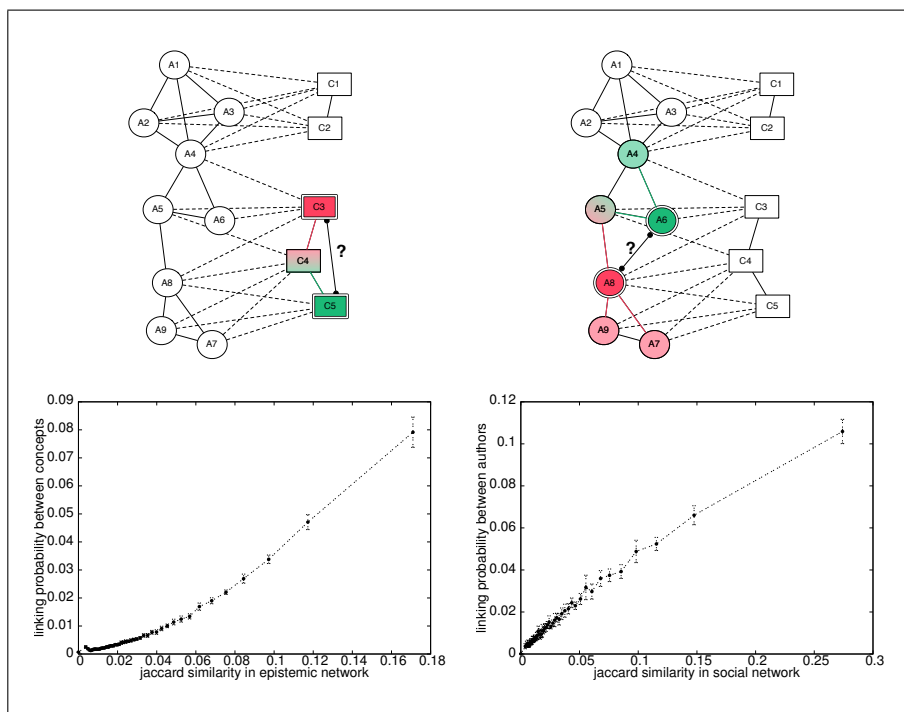
Figure 5. (Left) Linking probability between two concepts in the epistemic network in function of the Jaccard similarity of their neighbours. (Right) Linking probability between two authors in the social network in function of the Jaccard similarity of their neighbours. Values are averaged over all the considered years, and the error bars represent the 95% confidence level interval.
