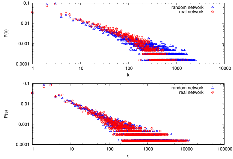
Figure 2. Real (red circles) and random (blue triangles) epistemic network distributions of degrees (up) and strengths (bottom)
