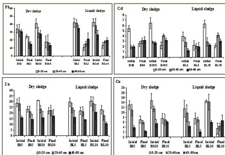
Figure 3: Comparison of Pb, Cd, Zn and Cu contents (mg/kg) in the soil before and after the last cutting of the Ray Grass.
