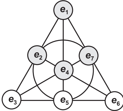
Figure 1: An illustration of the structure of \text{PG}(2,2) , the Fano plane, that provides the multiplication law for octonions (see, e. g., [4]). The points of the plane are seven small circles. The lines are represented by triples of circles located on the sides of the triangle, on its altitudes, and by the triple lying on the big circle. The three imaginaries lying on the same line satisfy Eq. (3).
