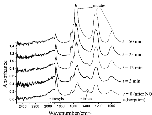
Fig. 8 Changes with time of FTIR spectra recorded on NO-preadsorbed \text{Ni}_{0.70}\text{Mn}_{2.30}\text{O}_{4+\delta} after introduction at -20^\circ\text{C} of pure \text{O}_2 ( P_{\text{O}_2} = 5 \times 10^4 \text{ Pa} ). Spectra are y -offset for clarity.
