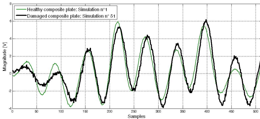
Figure 3: Impulse response of the healthy and damaged structure: composite plate model
