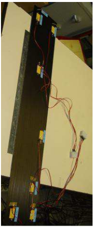
Figure 8: CLAS bounded with piezoceramic patches
