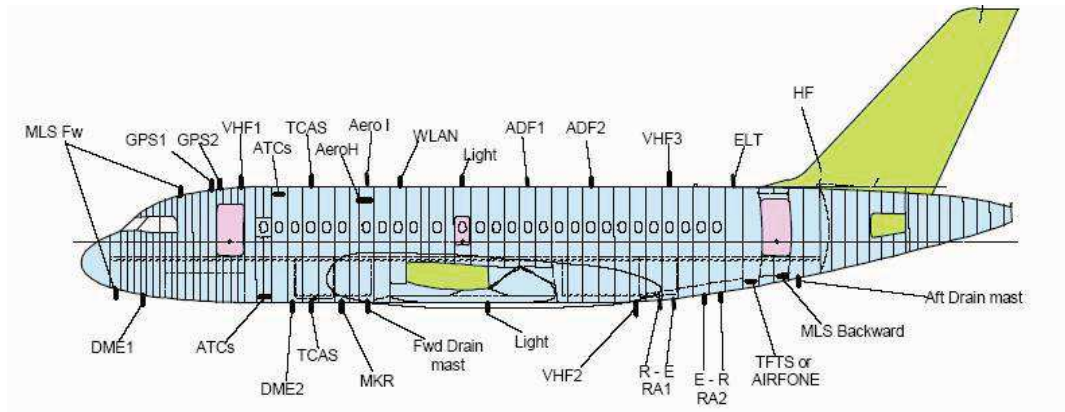
Figure 1: Antenna of the AIRBUS A318 [5]
