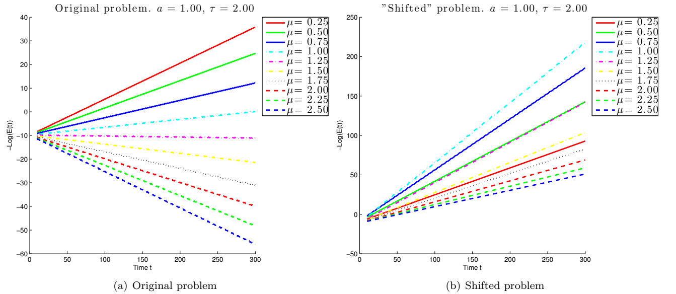
Figure 1: Energy (in -log scale) versus time: influence of \mu .
