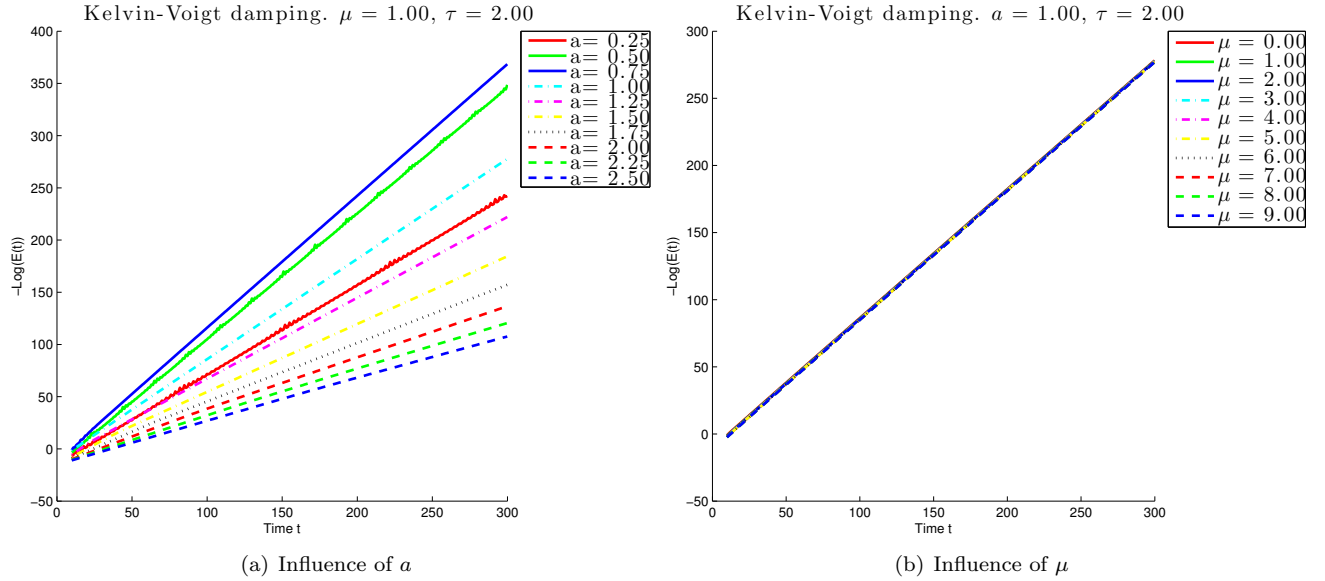
Figure 3: Energy (in -log scale) versus time.
