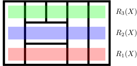
Figure 2: The gadget X with the regions R_1(X) , R_2(X) and R_3(X) .
