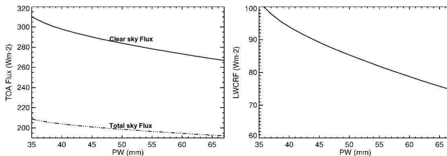
Fig. 6. Variation in TOA LW clear and total sky flux (left panel) and LWCRF (right panel) with Precipitable water (PW) over the Bay of Bengal region during the summer monsoon season using RRTM simulation.
