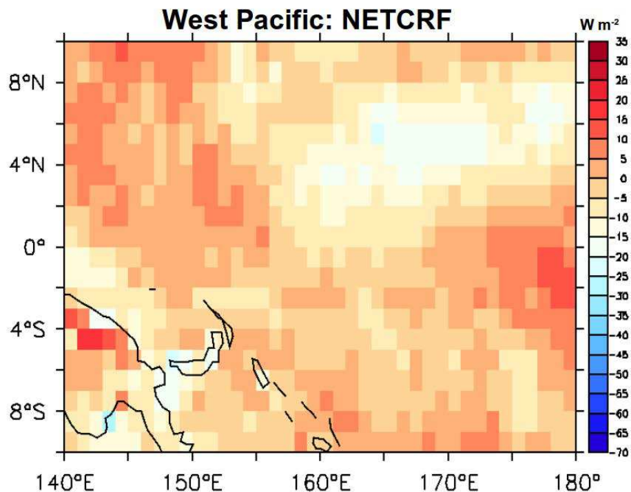
Fig. 8. Seasonal mean variation of NETCRF ( \text{W m}^{-2} ) over the West Pacific region during the March–April period (2002–2005). Color bar represents the NETCRF values in \text{W m}^{-2} .
