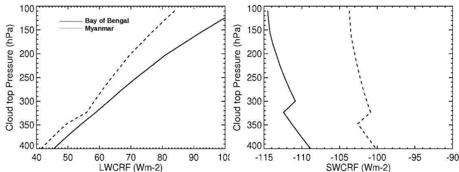
Fig. 5. Variation in LWCRF (left panel) and SWCRF (right panel) values with cloud top pressure for the Bay of Bengal (thick line) and Myanmar region (dashed line) respectively, estimated using RRTM.
