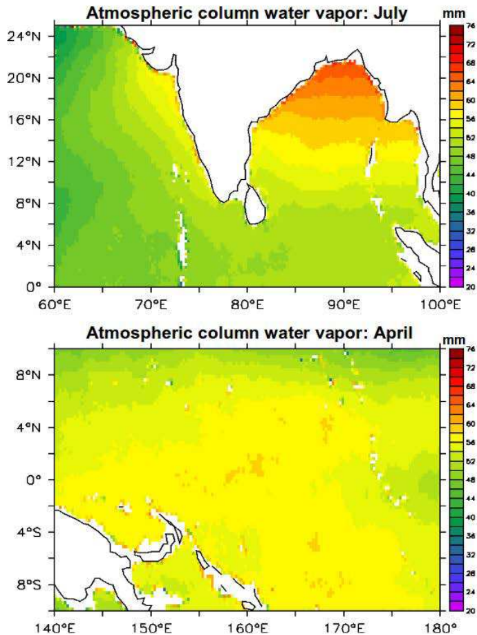
Fig. 9. Regional variation of monthly mean atmospheric water vapor (mm) from SSM/I over the Indian region (top panel) during the month of July and the West Pacific (bottom panel) during the month of April for the years 2002–2005.
