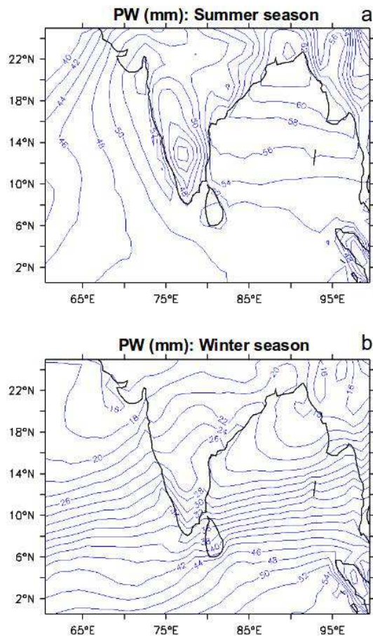
Fig. 7. Contour plots of seasonal mean variation of precipitable water (mm) content over the Indian region during the (a) summer monsoon season and (b) winter season for the period 2002–2005.
