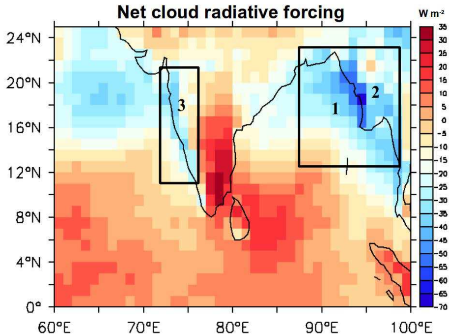
Fig. 3. Seasonal mean map of NETCRF over the Indian region during the summer monsoon season of 2002–2005. The negative NETCRF regimes (1) Bay of Bengal (2) Myanmar and (3) the Western Ghats (marked in boxes) are also shown. Color bar represents the NETCRF values in \text{W m}^{-2} .
