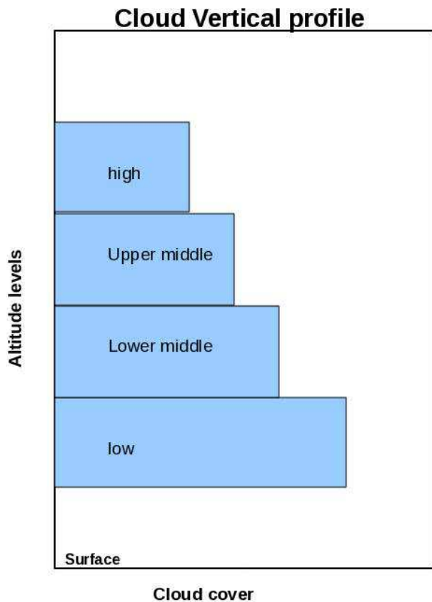
Fig. 1. Schematic of a typical vertical distribution of cloud fraction. Each shaded block represents the effective cloud amount for the respective cloud group estimated using the cloud fraction data and cloud overlap (maximum/random) scheme.
