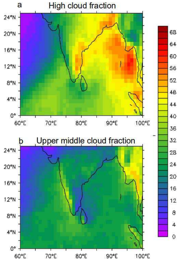
Fig. 4. Seasonal mean variation of (a) high cloud fraction (%) and (b) upper middle cloud fraction (%) over the Indian region during the summer monsoon season of 2002–2005. Color bar represents the mean cloud fraction in percentage.
