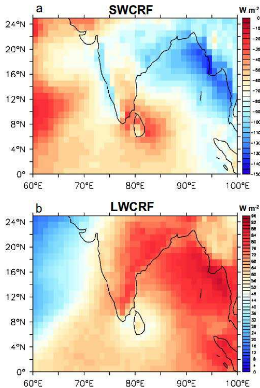
Fig. 2. Seasonal mean variation of (a) SWCRF and (b) LWCRF over the Indian region during the summer monsoon season of 2002–2005. Color bar represents the CRF values in \text{W m}^{-2} .
