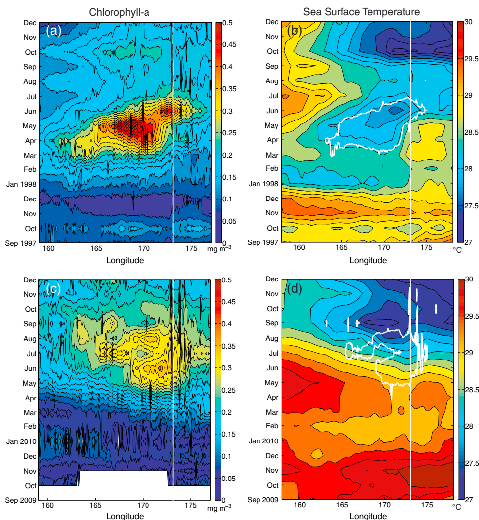
Figure 1. (a, c) 2^{\circ}\text{N} – 2^{\circ}\text{S} averaged SeaWiFS chl a ( \text{mg m}^{-3} ) and (b, d) SST ( ^{\circ}\text{C} ) from 158^{\circ}\text{E} – 178^{\circ}\text{E} for the 1998 El Niño/La Niña transition (Figures 1a and 1b) and the 2010 El Niño/La Niña transition (Figures 1c and 1d). The vertical white lines denote the approximate location of the Gilbert Islands. Black contour intervals are approximately 0.03 \text{ mg m}^{-3} (Figures 1a and 1c) and 0.3 \text{ }^{\circ}\text{C} (Figures 1b and 1d). The bloom domain ( >0.3 \text{ mg m}^{-3} ) is overlaid in Figures 1b and 1d as a white line.
