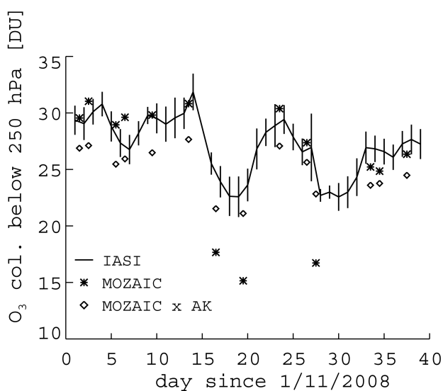
Fig. 8. Time series of O 3 tropospheric (surface–250 hPa) columns near Hyderabad from 1 November 2008 until 10 December 2008 from (asterisque) MOZAIC (diamonds) MOZAIC convolved with IASI Averaging Kernels (solid line) IASI-SOFRID coincident ( \pm 1.5^\circ , \pm 12 h) pixels. Error bars correspond to IASI 1\sigma standard deviations.
