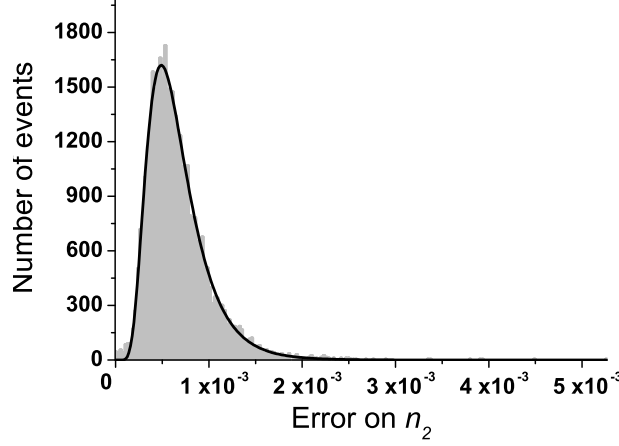
FIG. 5: Distribution of the uncertainties \Delta n_2 over all the simulated guides, fitted by a lognormal law.
