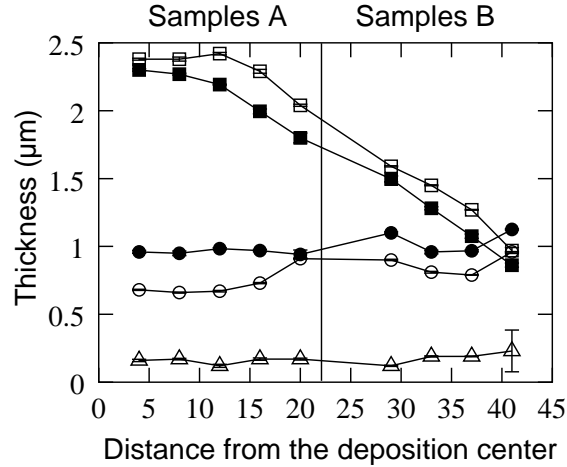
FIG. 12: Evolution of the thicknesses of the different layers of the three layer samples A_r , B_r ( d_1 : \square , d_2 : \circ , d_3 : \triangle ) and the two layer samples A_l , B_l ( d_1 : \blacksquare , d_2 : \bullet ).
