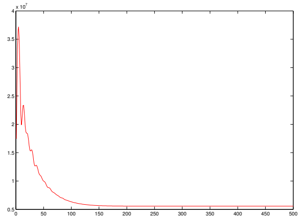
(a) The value of the functional is decreasing during the convergence of the algorithm.
