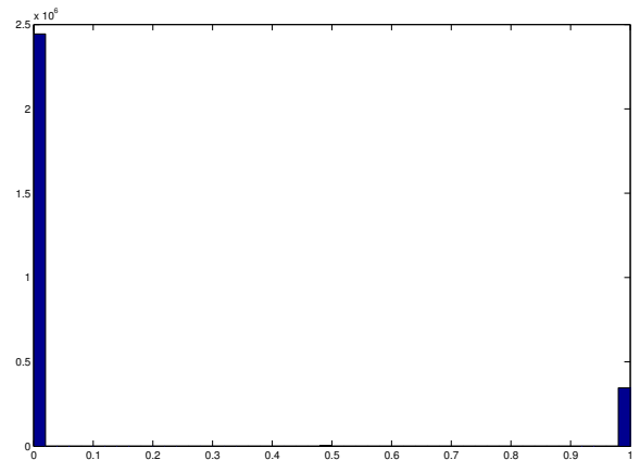
(b) Histogram of W at convergence of the algorithm.
